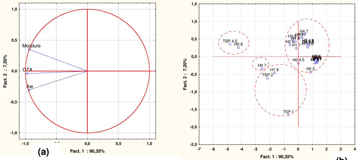
Figure 4: Correlation drawn between the f1-f2 factorial of the principal components analysis and the chemical parameters (a) and the individuals (b) deriving from the cowpea samples studied
