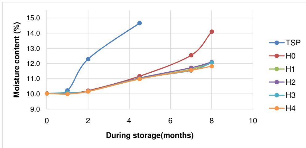
Figure 1: Evolution of moisture content during storage
