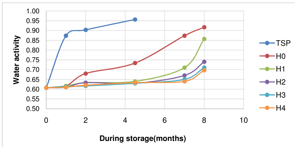
Figure 2 : Evolution of water activity during storage
