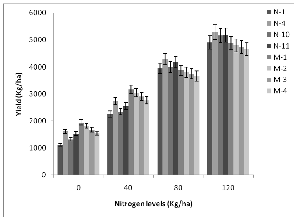
224 Fig. 4. Effect of N rate on yield component of eight rice varieties grown at four levels of nitrogen 225 treatment (Means of three replicates \pm SE). LSD (0.05) V = 99.68, T = 70.48.
