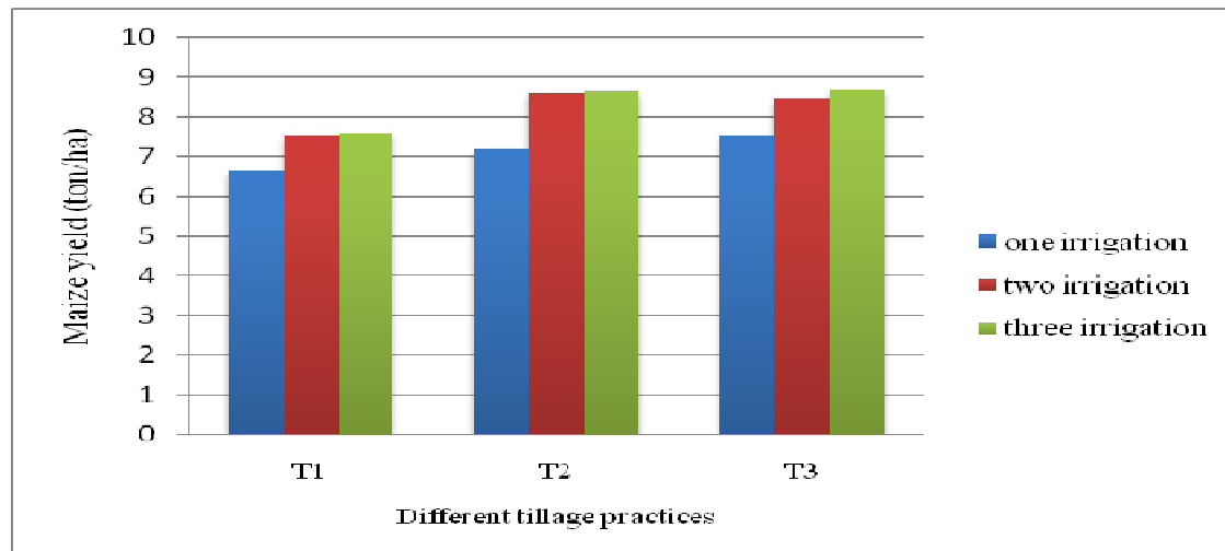
Fig. 2 Effect of irrigation on maize yields with different tillage practices.
