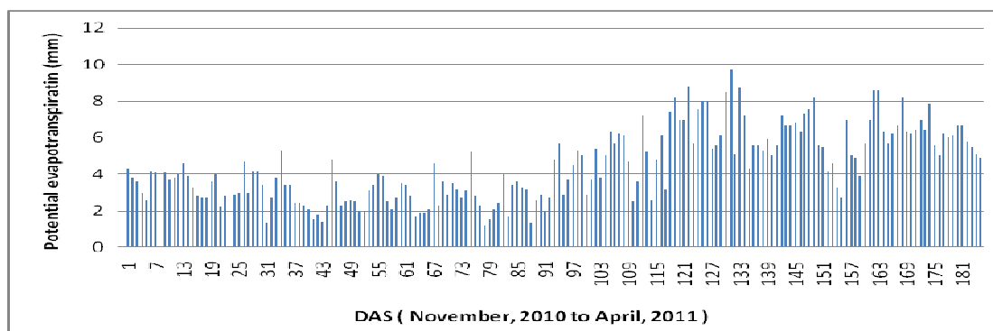
Fig. 1 Daily potential evapotranspiration (ET o ) during experiment season.
