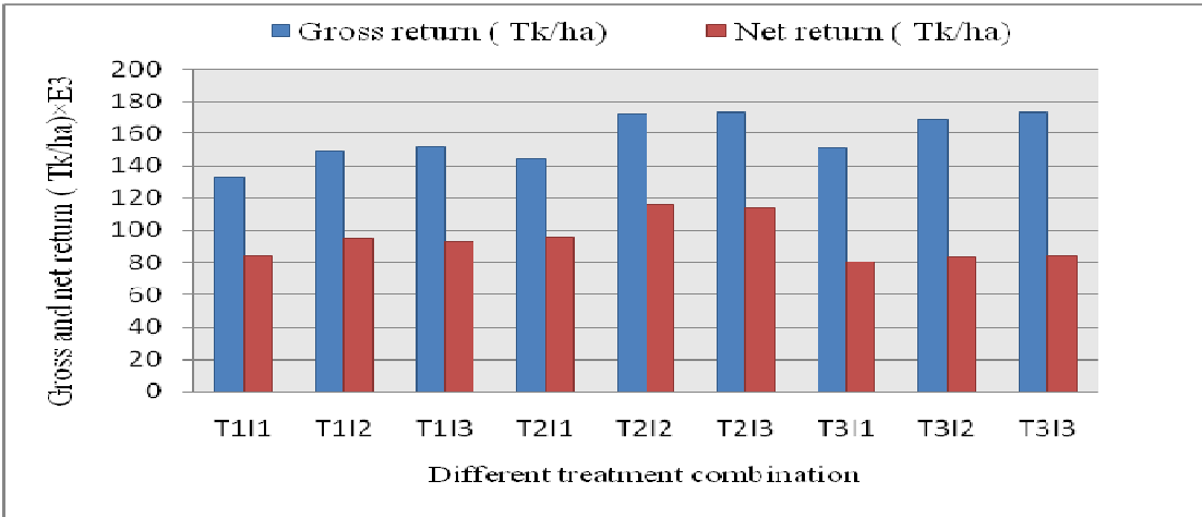
Fig.5 Gross and net return of maize cultivation with different treatment combination
