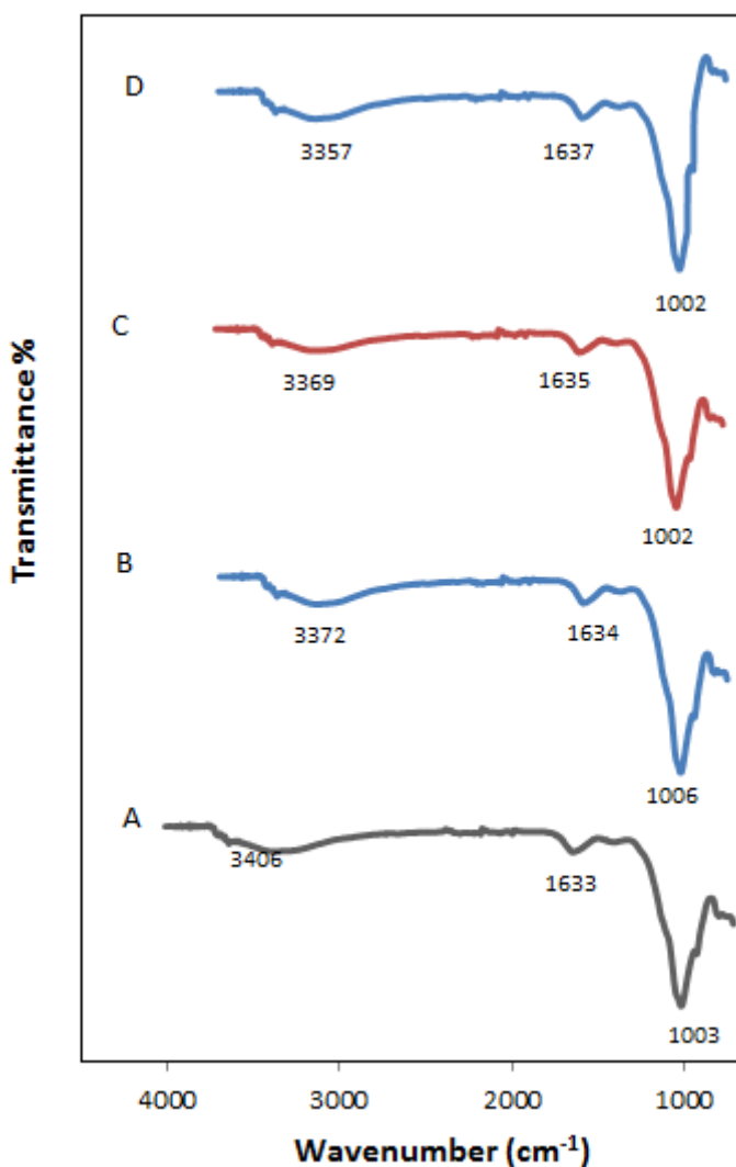
Figure 2 FTIR spectra of (A) soil, (B) soil with chlorsulfuron, (C) soil with Cu (II), and (D) soil with chlorsulfuron and Cu (II).
