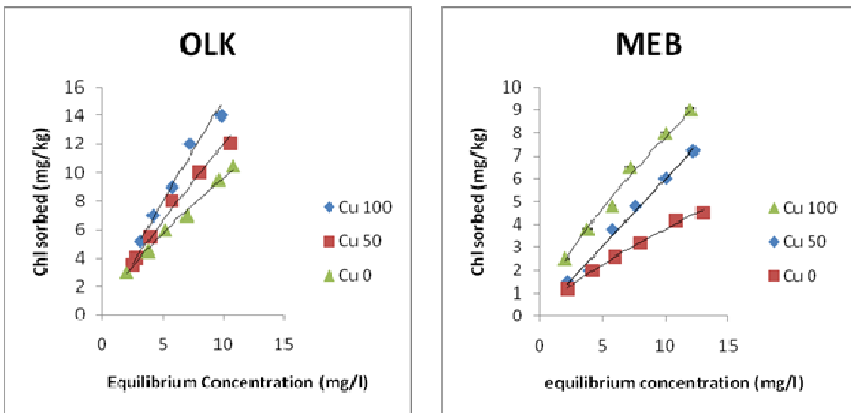
Figure 1 Sorption isotherms of chlorsulfuron in Mau Central (MC), Mau East A (MEA), Olokurto (OLK) and Mau East B (MEB) soils in presence and absence of Cu (II).
