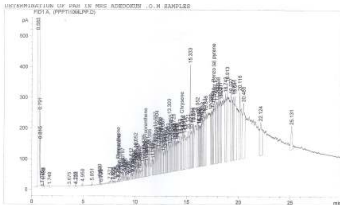
Figure 1f: Chromatogram of Poly cyclic aromatic Hydrocarbon Profile of Crude oil polluted cotton with Pleurotus pulmonarius
