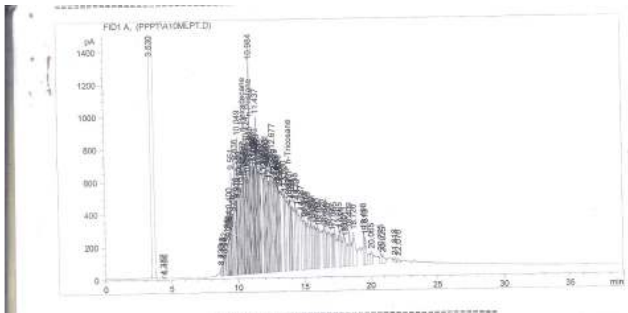
Figure 1c: Chromatogram of Aliphatic Hydrocarbon Profile of Crude oil polluted cotton with Pleurotus tuber-regium
