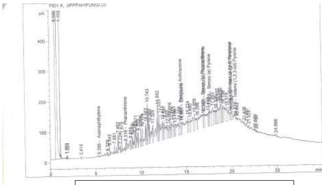
Figure 1h: Chromatogram of Poly cyclic aromatic Hydrocarbon Profile of Crude oil polluted cotton with Lentinus squarrosulus
