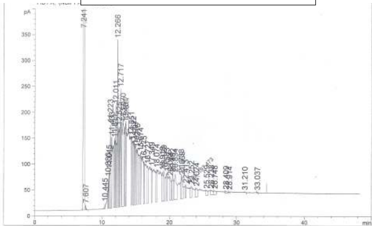
Figure 1c: Chromatogram of Aliphatic Hydrocarbon Profile of Crude oil polluted cotton with Pleurotus tuber-regium
