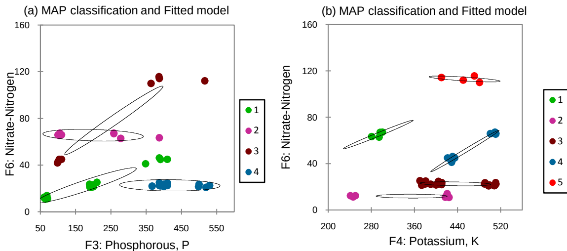
Fig. 10. Scatter plots of 4 two-dimensional Gaussians of phosphorous on Nitrate-Nitrogen (a) (b) and a 5 two-dimensional Gaussian of potassium on Nitrate-Nitrogen with full covariance matrices. Best model for both cases was the EEV
