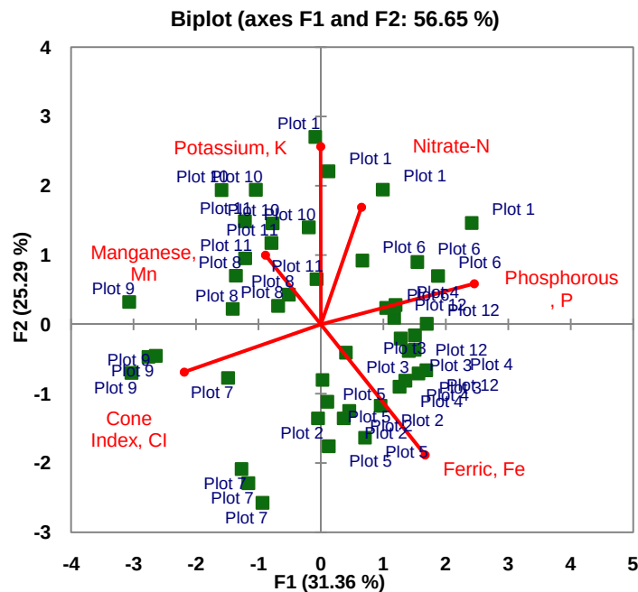
Fig. 3. Biplot generated by the principal component analysis for some soil nutrients and CI distributed within the different plots of the sandy loam soil ( EutricLeptosol )
