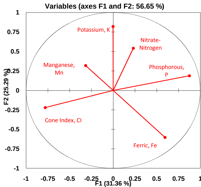
Fig. 2. Loading plots of principal components analysis on soil nutrients: Nitrate-N, P, K, Fe, Mn as well as soil penetration resistance measured as Cone Index, CI
