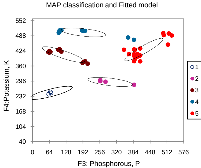
Fig. 9. Scatter plots of 5 two-dimensional Gaussians of phosphorous on potassium with full covariance matrices. Best model was the EEV (Equal volume, Equal shape and Variable orientation)
