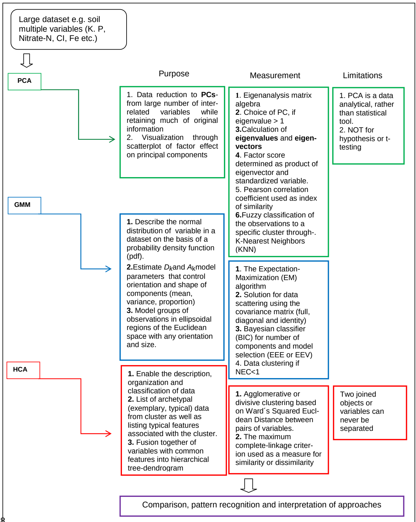
Fig. 1. Diagrammatic representation of the proposed multivariate analysis using the PCA, HCA and GMM approach on soil variables of EutricLeptosol
