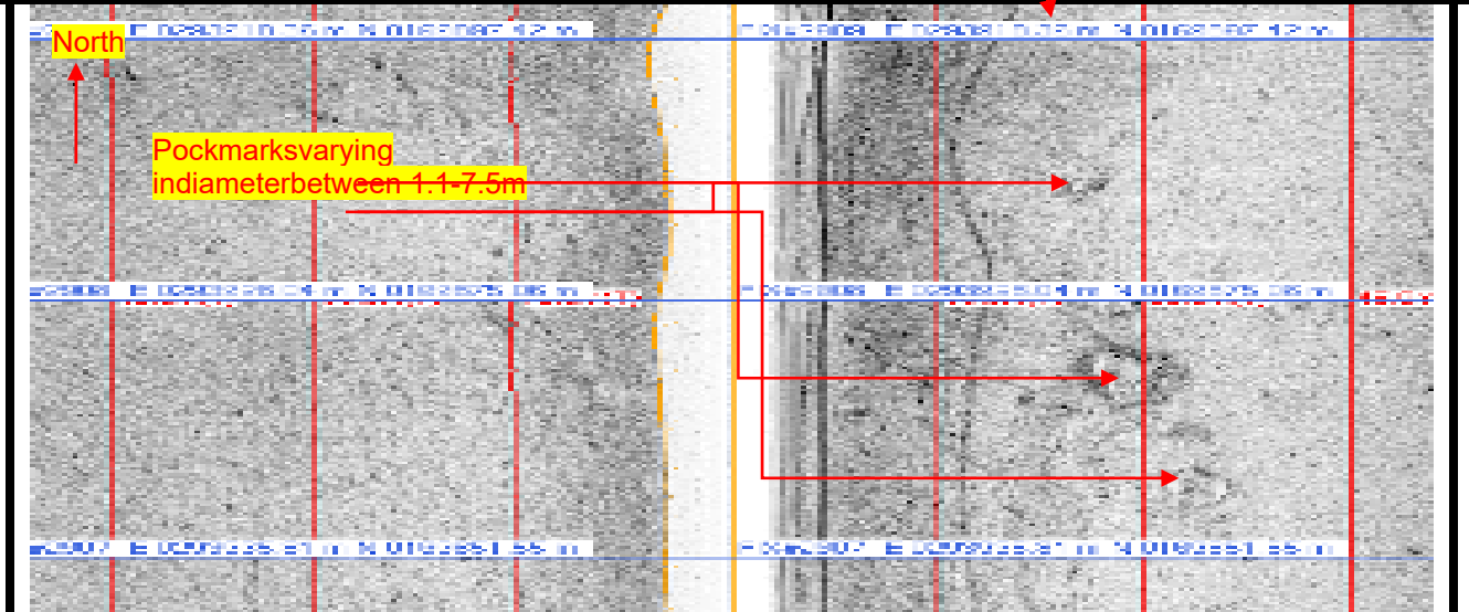
Figure 11: SSS Data extract showing Pockmarks on seafloor of study area study area .....
