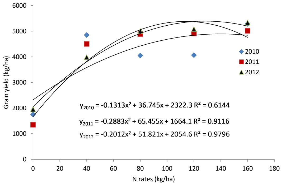
Figure 1. Trend analysis for grain yield for 2010, 2011 and 2012 cropping
