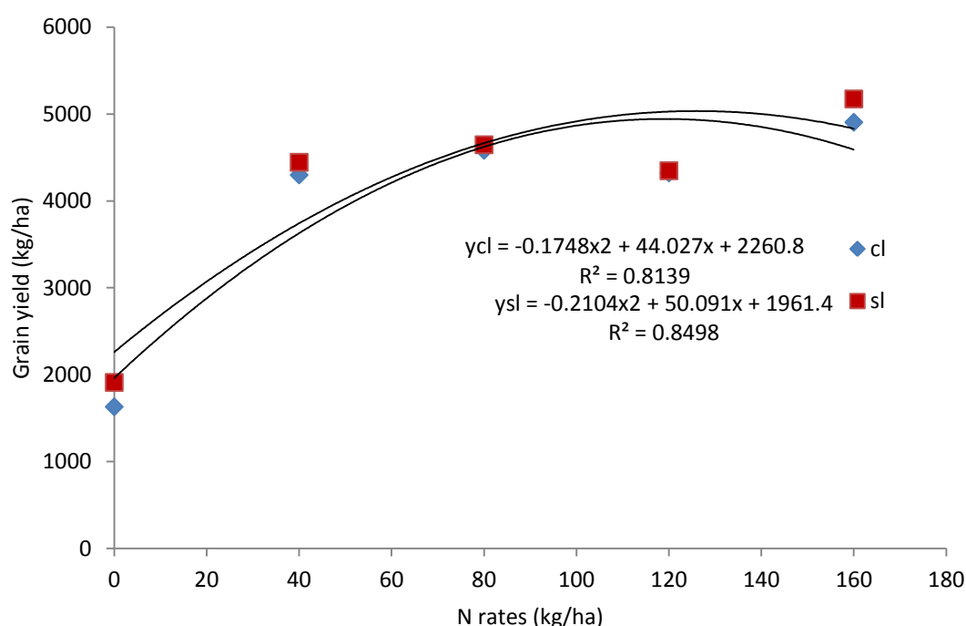
Figure 2. Trend analysis for grain yield on Clay-loam and Sandy-loam soils
