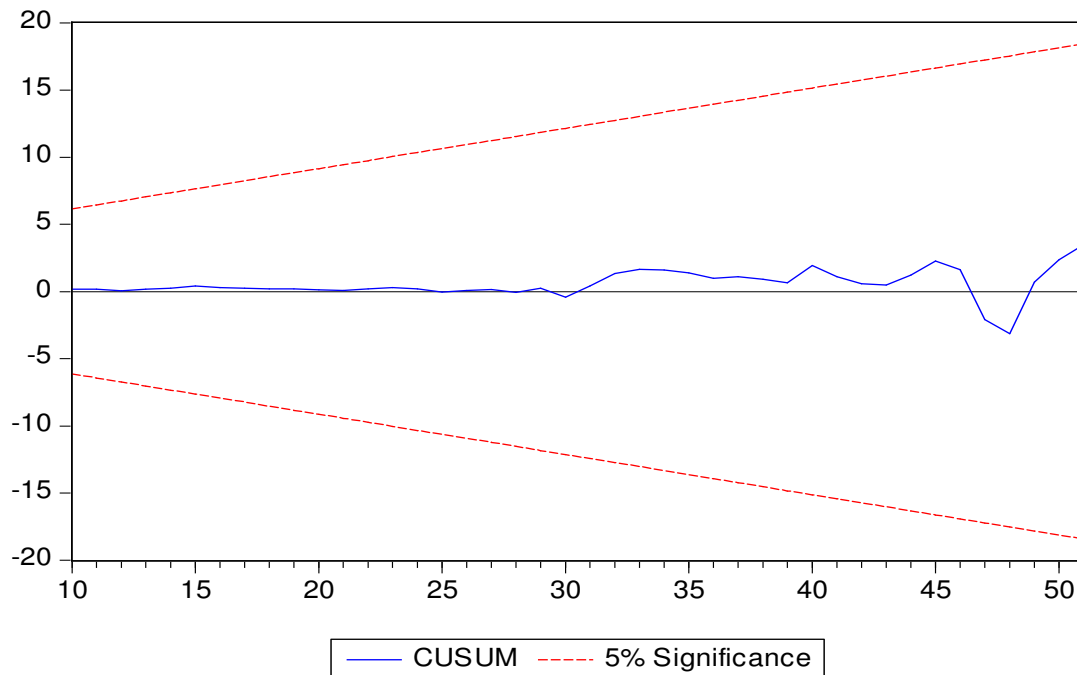
Fig. 1. Plot of CUSUM for the estimated ECM model
