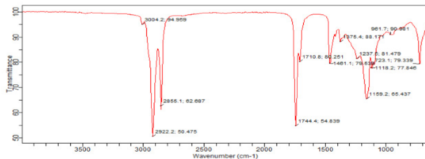
Fig. 1. FTIR spectrum of the PWCPO
