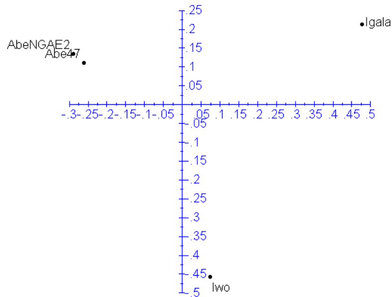
314 Figure 3.3.1: Factorial analysis of the okra accessions
