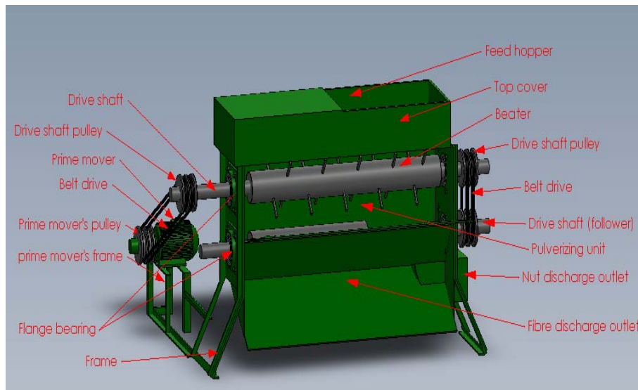
Fig. 3b. 3-D drawing of the constructed machine
