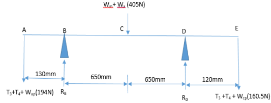
Fig. 2. The auger shaft showing forces acting on it
