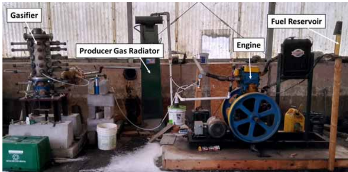
Fig. 5. CERF Gasifier Genset System [26]
