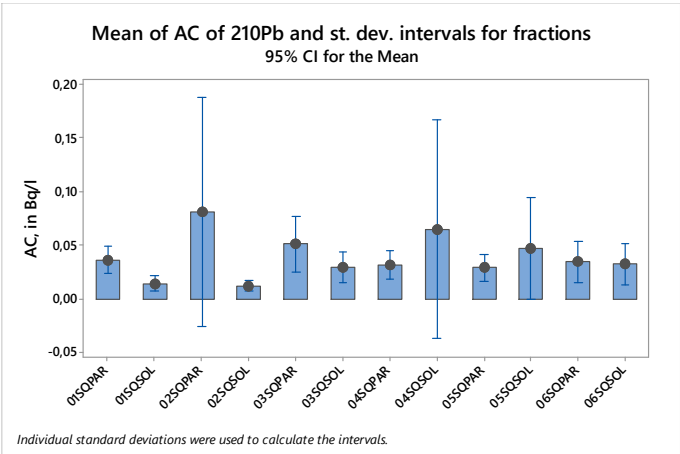
Figure 2. Mean and intervals (st.dev.) for AC of 210 Pb in soluble (SOL) and particulate (PAR) fractions in surface water of Santa Quitéria region.
