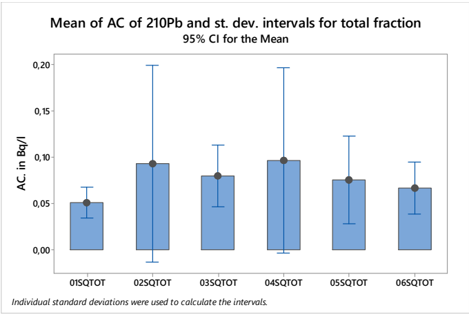
Figure 3. Mean and intervals (st.dev.) for AC of 210 Pb in total fractions (TOT) in surface water of Santa Quitéria region.
