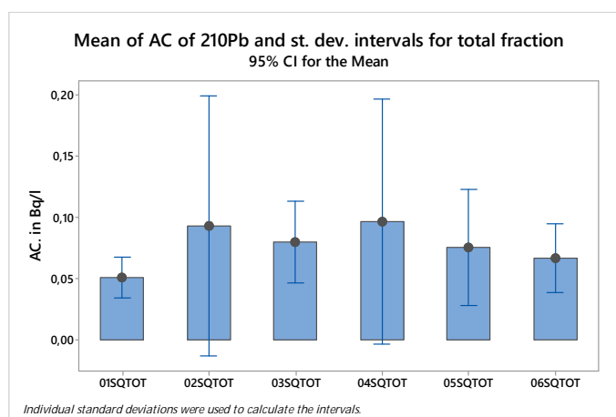
Figure 3. Mean and intervals (st.dev.) for AC of ^{210}\text{Pb} in total fractions (TOT) in surface water of Santa Quitéria region.
