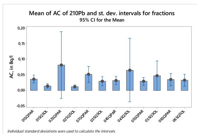
Figure 2. Mean and intervals (st.dev.) for AC of ^{210}\text{Pb} in soluble (SOL) and particulate (PAR) fractions in surface water of Santa Quitéria region.
