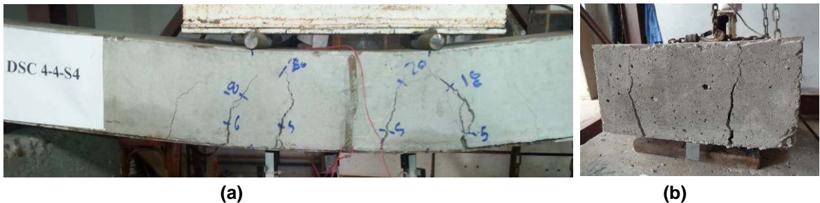
Fig. 10. View after failure load of the specimen DSC 4-4-S4 with wide crack in concrete (a), and close up view of the right side corner showing longitudinal cracks in concrete (b).
