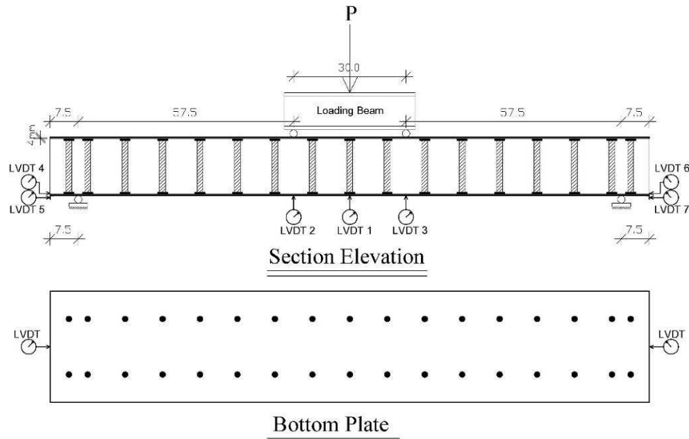
Fig. 5. The arranged of LVTDs
