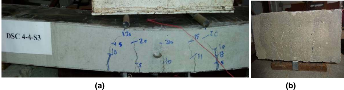
Fig. 9. View after failure load of the specimen DSC 4-4-S3 with wide crack in concrete (a), and close up view of the right side corner showing longitudinal cracks in concrete (b).
