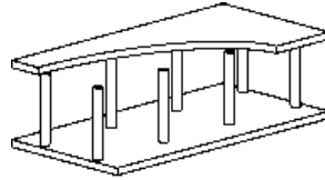
(b) Bi-Steel sandwich construction (Bi-Steel).
