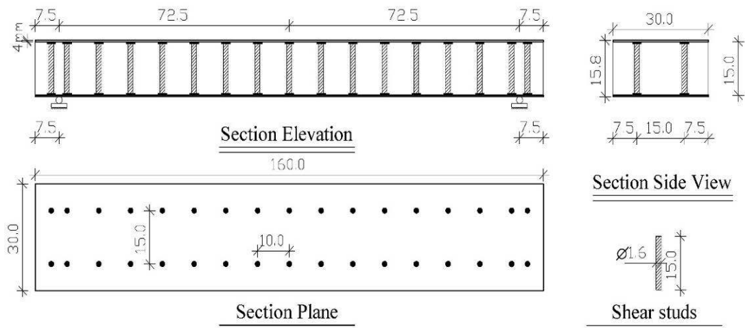
127 Fig. 3. A typical layout of studs and the relevant details of DSC 4-4-S2.
