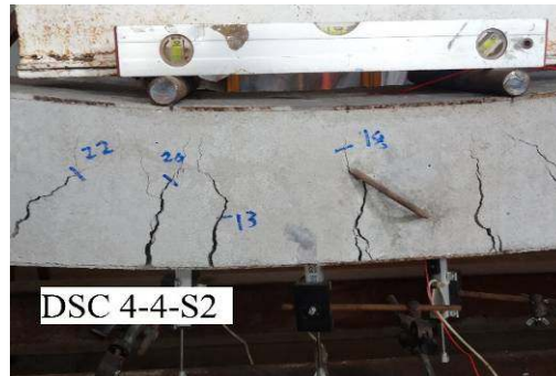
(a) Wide flexural crack in concrete core.
