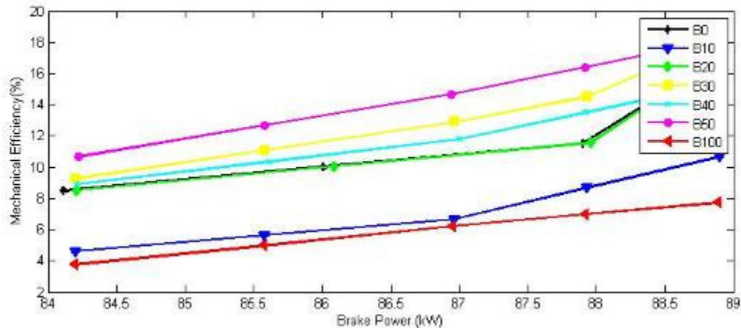
Figure.1 Variation of mechanical efficiency with brake power
