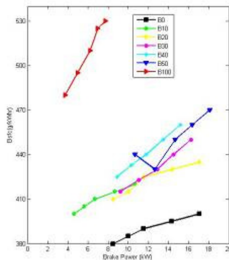
Figure. 2 Variation of brake specific fuel consumption with brake power
