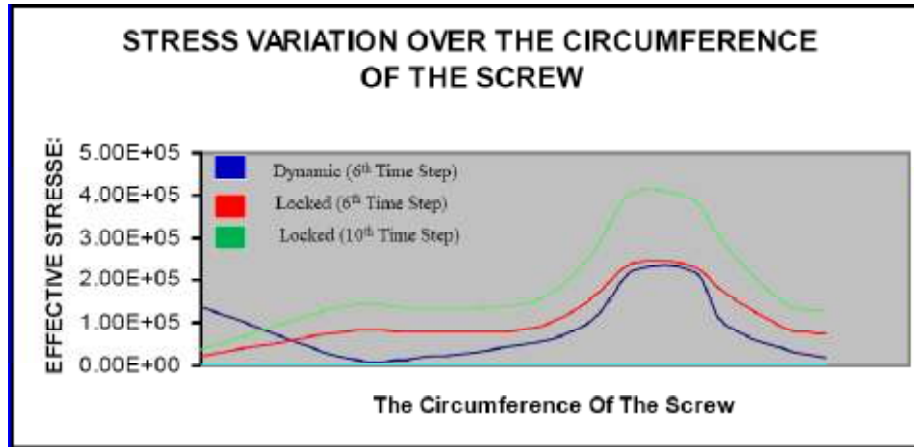
Figure 6: Stress variation (in Pascal) over the circumference of the screw at different time steps for Dynamic and Locked plates in torsion.
