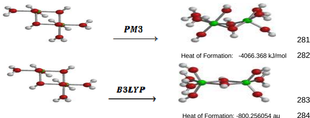
Fig. 11 : (101) surface Optimized geometrical formula in acidic medium.
