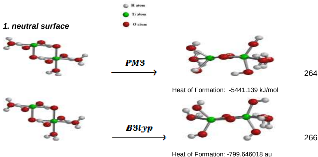
Fig. 9 : (101) surface Optimized geometrical formula in neutral medium .
