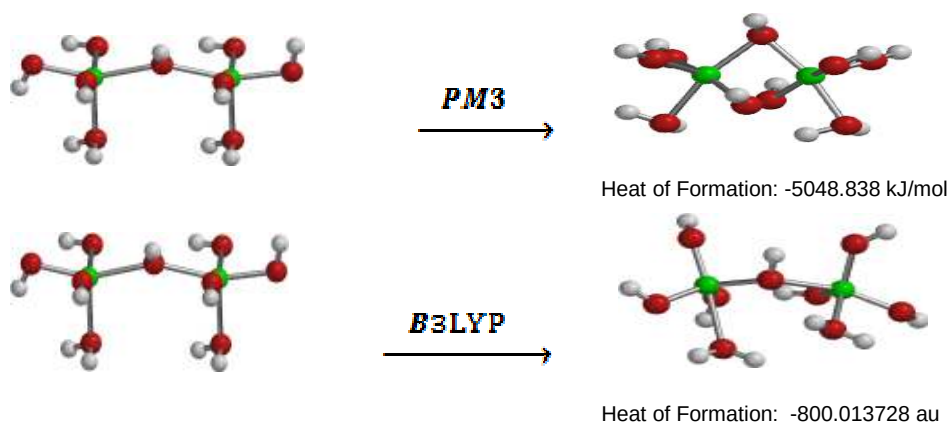
247 Fig. 8 : (001)surface Optimized geometrical formula in acidic medium .
