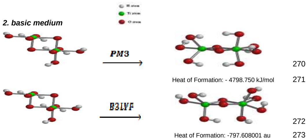
Fig. 10 : (101) surface Optimized geometrical formula in basic medium .
