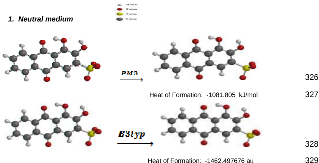
Fig. 12 :ARS pollutant Optimized structure in neutral medium by(PM3)(B3LYP) .
