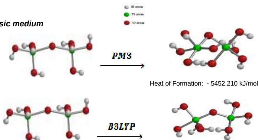
234 Fig. 6 : (001)surface Optimized geometrical formula in neutral medium . 235
