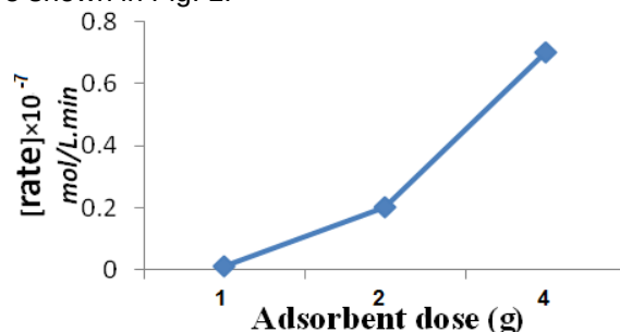
Fig.2 Effect of photo catalyst dose on ARS degradation rate. experimental parameters: contact time, t (15 min), initial concentration of dye (20 ppm), temp. (30 ^{\circ}\text{C} ) and solution volume 25 ml .
