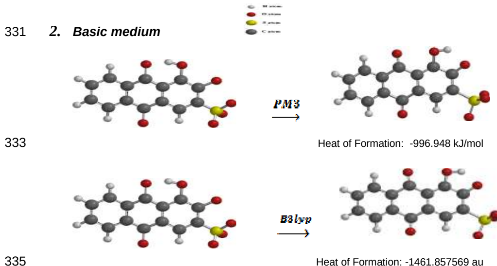
Fig. 13 :ARS pollutant Optimized structure in basic medium by(PM3)(B3LYP).
