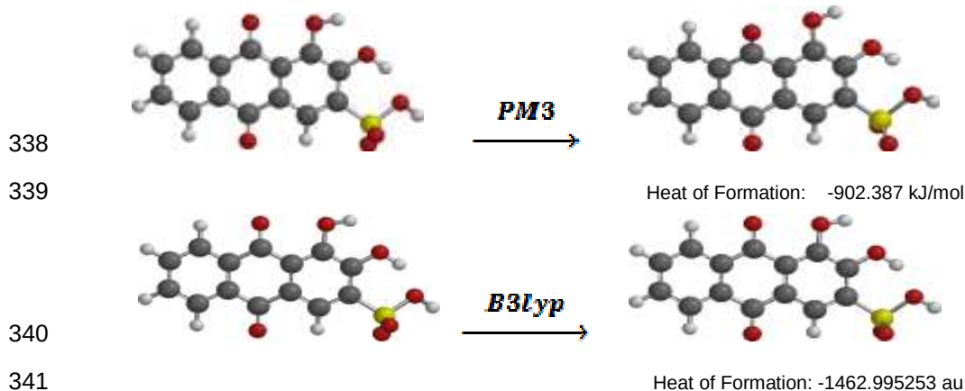
Fig. 14 :ARS pollutant Optimized structure in acidic medium by(PM3)(B3LYP).
