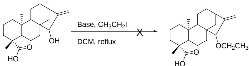
Scheme 3.4 Attempted route for ether formation.
