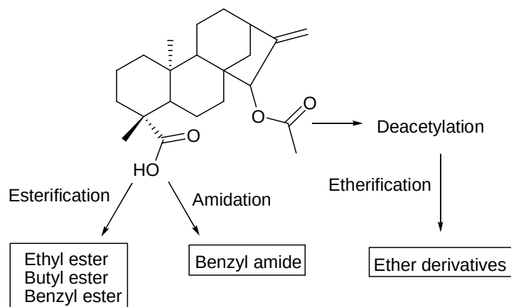
47 Scheme 1.1 Synthetic strategies and proposed modifications on xylopic acid
