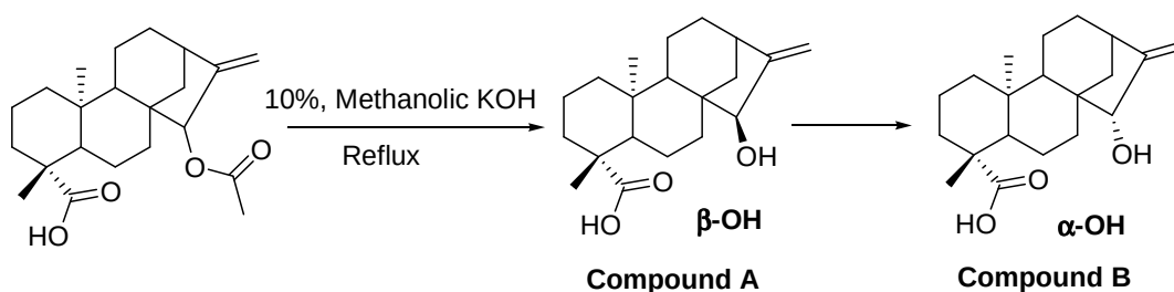
Scheme 3.3 Epimerization of deacetyl xylopic acid
