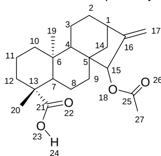
Fig.3.1 Structure of xylopic acid showing atom numberings
