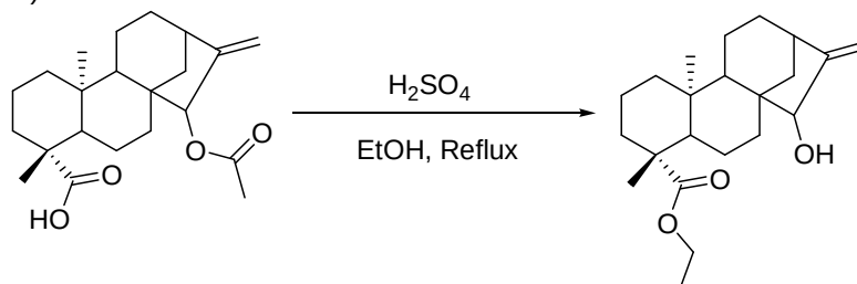
Scheme 3.1 Proposed reaction for acid catalysed ethyl ester formation.
