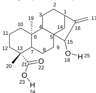
Fig. 3.2 Structure of deacetyl xylopic acid showing atom numberings.
