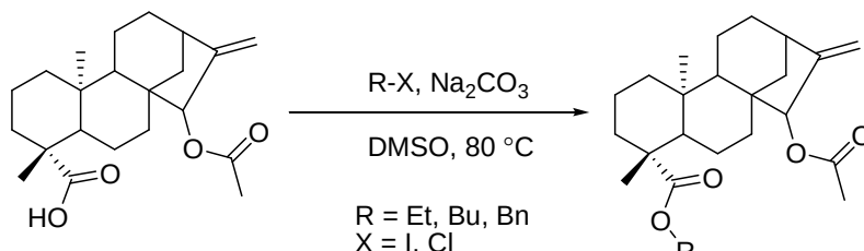
Scheme 3.2 : Base mediated esterification of xylopic acid
