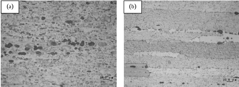
Fig.2 Microstructure of alloys before and after homogenization (a) before homogenization, (b) after homogenization
