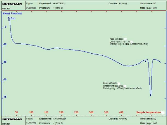
Fig.1 DSC curve of Al-5.2%Zn-2.3%Mg alloy
