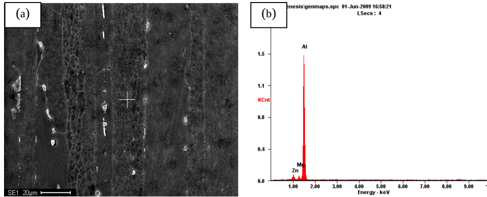
Fig.3 Composition scanning of matrix after homogenization
