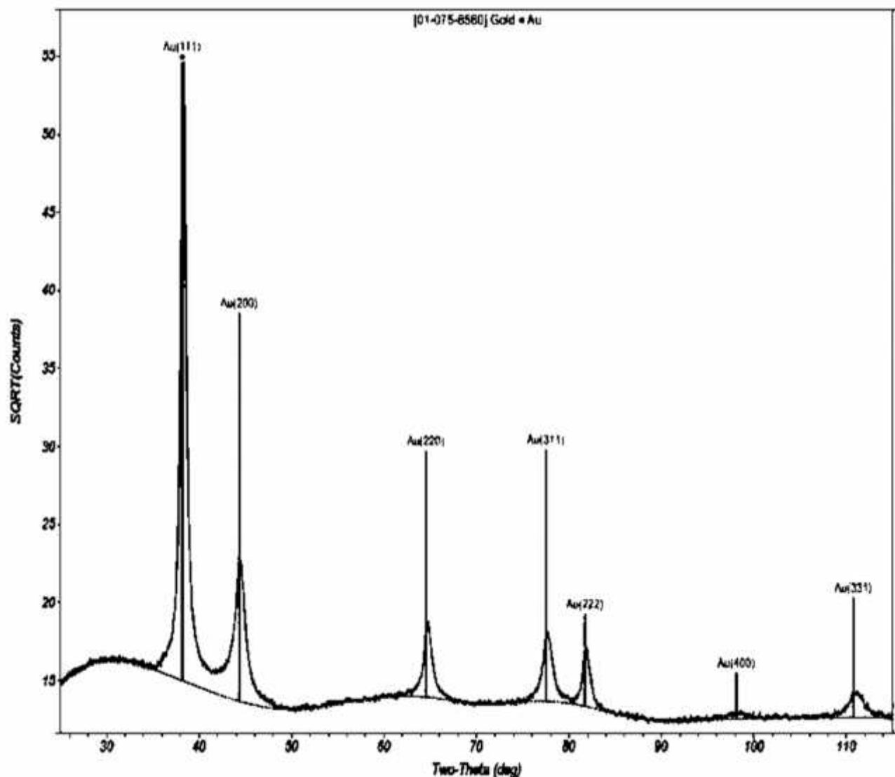
Figure 2 X-ray diffraction (XRD) patterns of the gold nanoparticles synthesized by chemical method from precipitated gold using NaCN and cyanide solution from cassava
