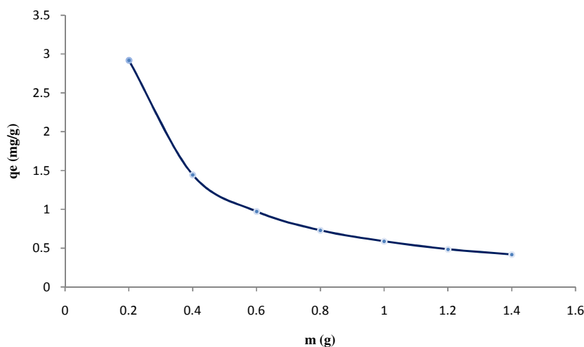
Fig. 3. Influence of the mass of pillared clay on Gallic acid adsorption.
