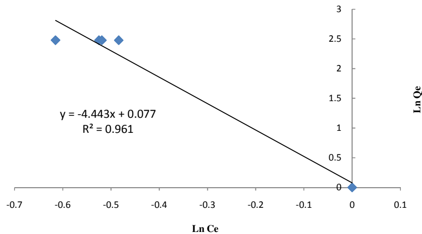
Fig. 7. Freundlich plot for the Gallic acid uptake by pillared clay mineral from Boboyo
