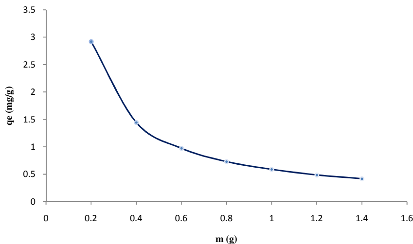
Fig. 3. Influence of the mass of pillared clay on Gallic acid adsorption.
