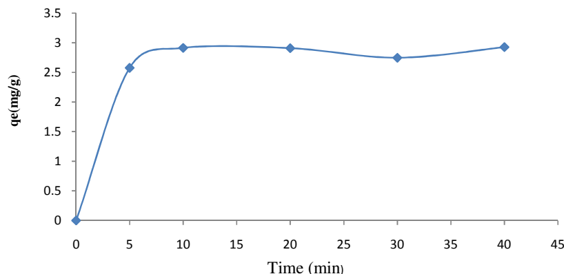
Figure2. Kinetics study for Gallic acid uptake by pillared clay from Boboyo.
