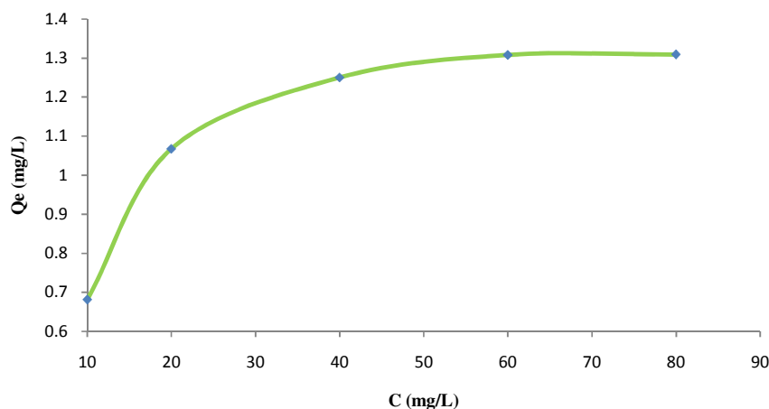
Fig. 4. Effect of solution concentration on adsorption of Gallic acid onto pillared clay
