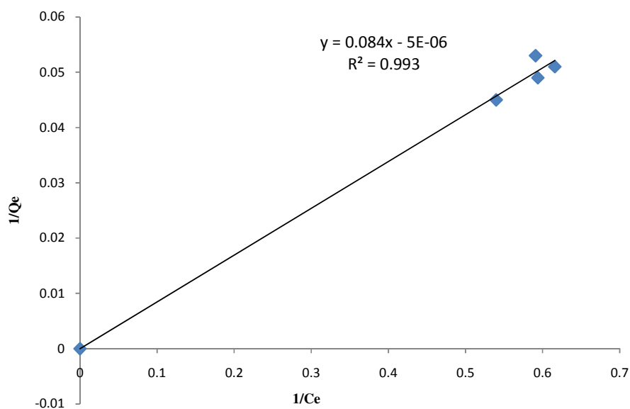
Figure. 6. Langmuir plot for the Gallic acid uptake by pillared clay mineral from Boboyo
