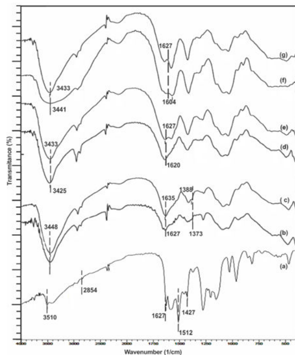
149 Fig. 3. FTIR spectra of curcumin (a), AK-0 (b), AK (c), ACaK-0 (d), ACaK (e), KACa-0 (f) and 150 KACa (g).
