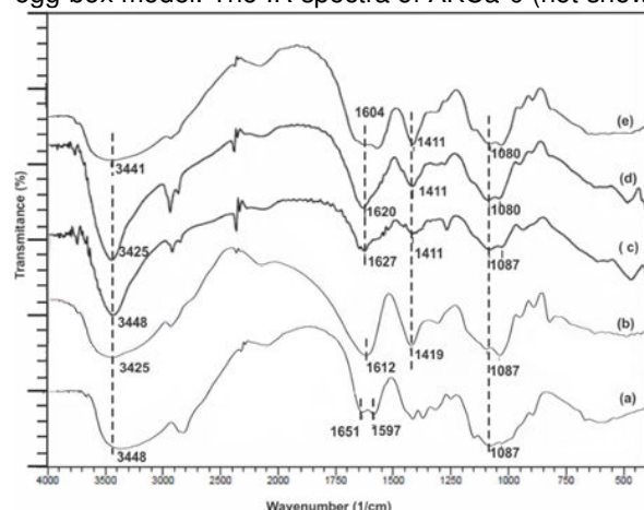
Fig. 2. FTIR spectra of chitosan (a), sodium alginate (b), AK-0 (c), ACaK-0 (d) and KACa-0 (e).
