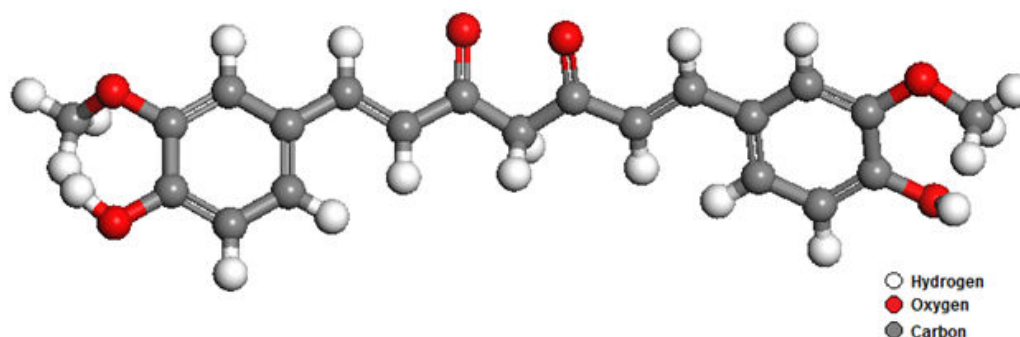
Fig. 1. Chemical structure of curcumin.
