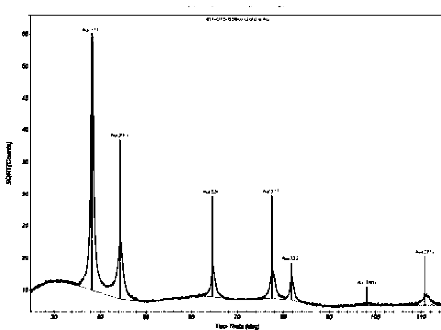
Figure 1 X-ray diffraction (XRD) patterns of the gold nanoparticles synthesized by chemical method from precipitated gold using NaCN and cyanide solution from cassava
