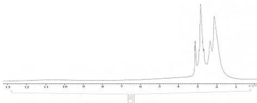
231 Figure 5. ^1\text{H} NMR spectrum of PAA/DOX composite
