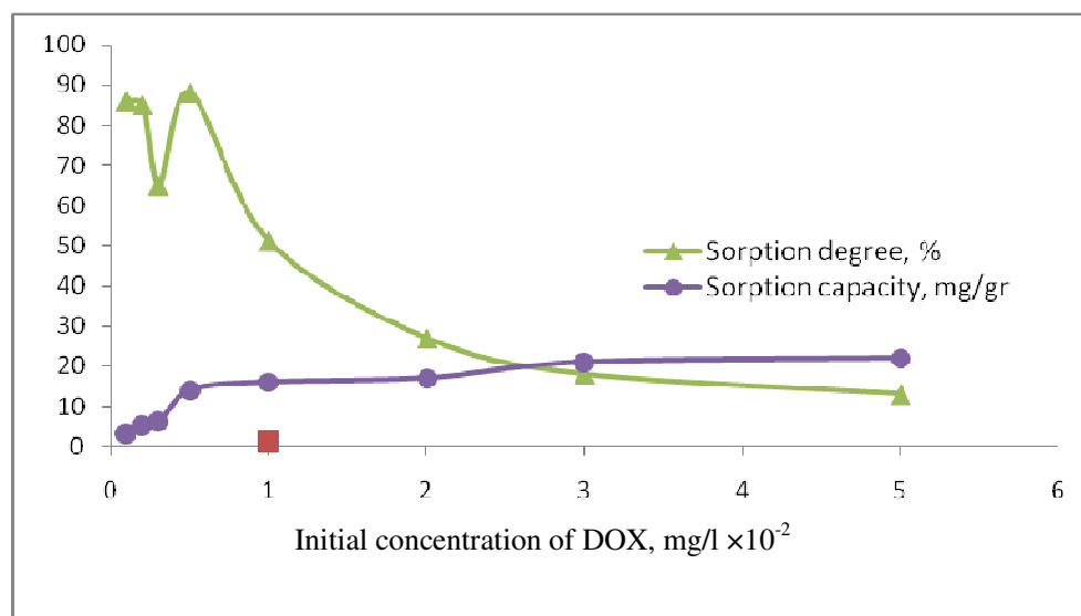
Figure 2. Dependence curves of sorption capacity of 10% cross-linked polyacrylic acid for doxorubicin and dependence curves of sorption degree on starting concentration of antibiotic
