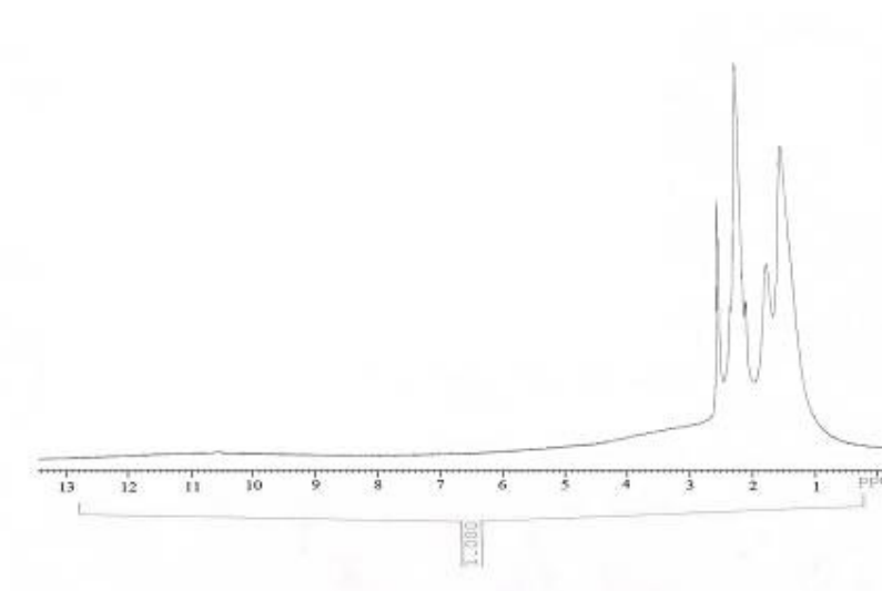
228 Figure 4. ^1\text{H} NMR spectrum of PAA
