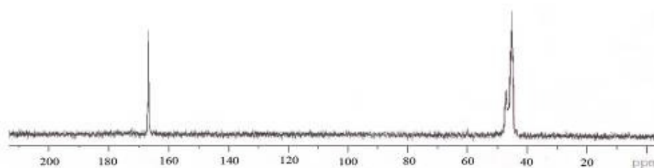
Figure 7. ^{13}\text{C} NMR spectrum of PAA/DOX composite
