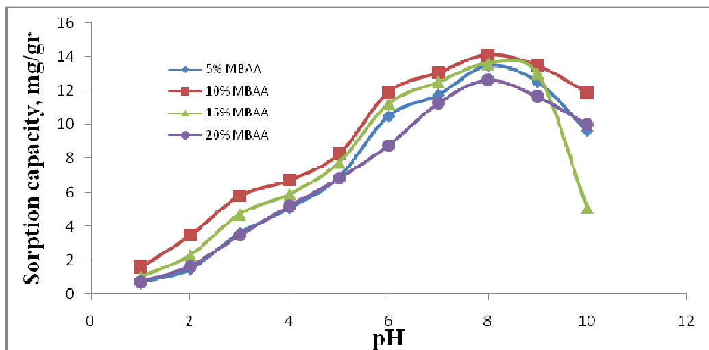
Figure 1. Dependence curves of pH environment of sorption capacity for DOX of PAA based gel cross-linked in different % ratio with MBAA.
