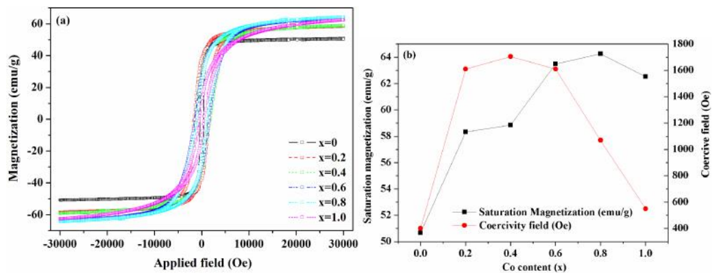
Figure 9. (a) Room temperature magnetic hysteresis loops of the \text{Ni}_{1-x}\text{Co}_x\text{Fe}_2\text{O}_4 nanoparticles and (b) variations of saturation magnetization and coercivity as a function of Co content.
