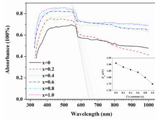
394 Figure 4. Absorbance spectra of the \text{Ni}_{1-x}\text{Co}_x\text{Fe}_2\text{O}_4 nanoparticles. The inset is the plot 395 of band gap ( E_g ) vs. Co content ( x ).
