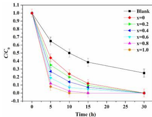
412 Figure 7. Concentration variations of malachite green aqueous solutions containing 413 \text{H}_2\text{O}_2 (concentration equals to 10 ml/l) on the \text{Ni}_{1-x}\text{Co}_x\text{Fe}_2\text{O}_4 nanoparticles 414 with irradiation time of sunlight.
