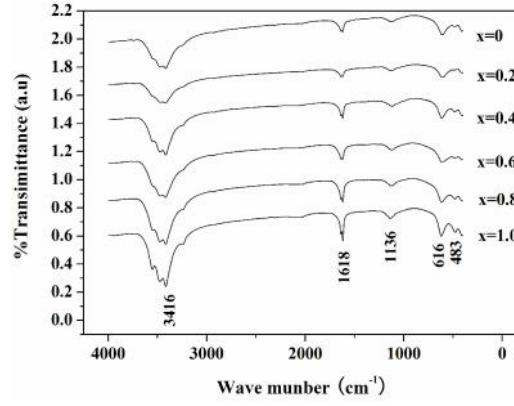
392 Figure 3. FTIR spectra of the \text{Ni}_{1-x}\text{Co}_x\text{Fe}_2\text{O}_4 nanoparticles.
