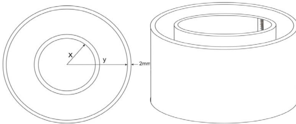
Figure 2: double ring infiltrometer plan and assembling
