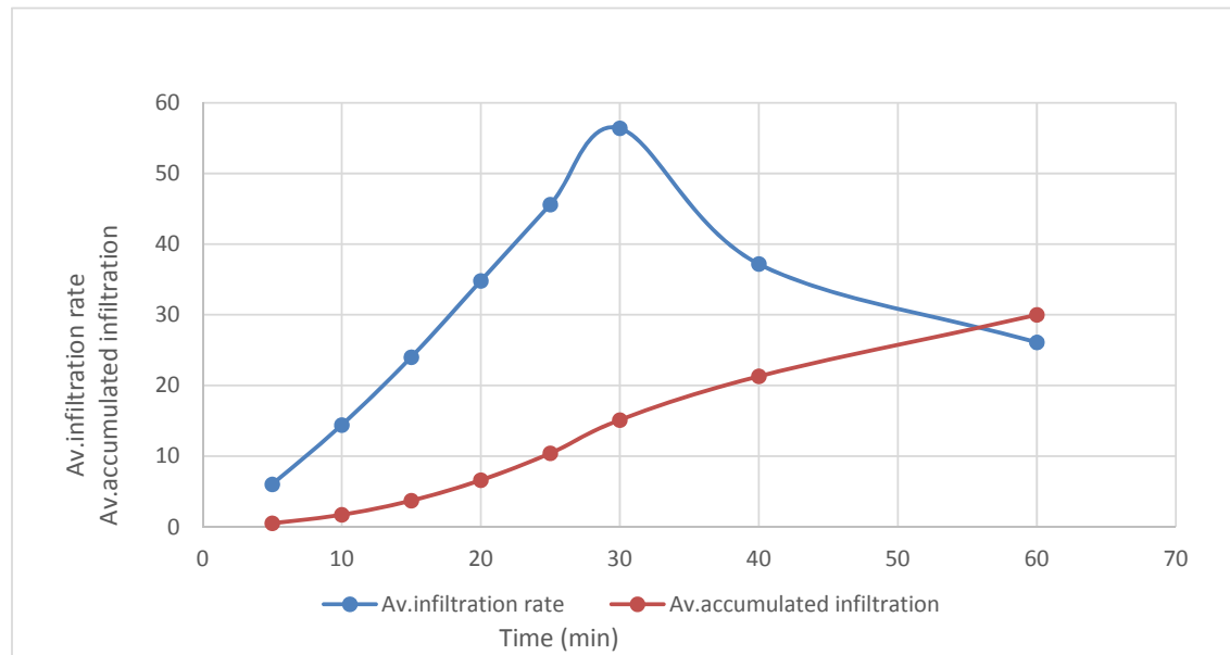
Figure 6: Graph of infiltration rate for location 2
