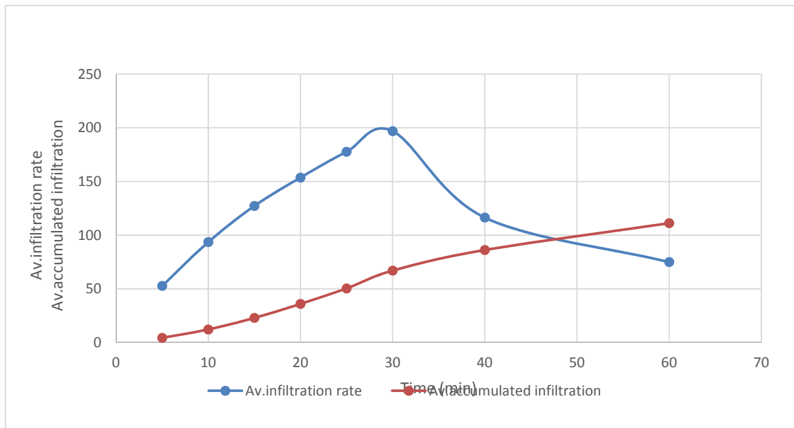
134 Figure 5: Graph of infiltration rate for location 1
