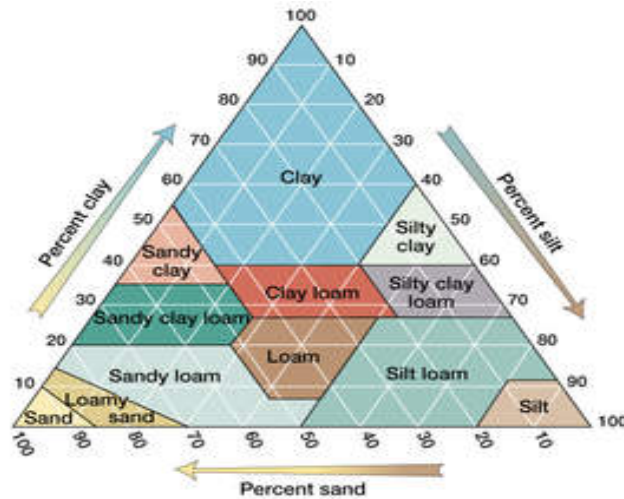
Figure 4: Soil Texture Triangle
