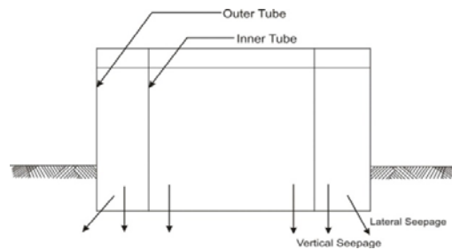
Figure 1: Section double ring infiltrometer
