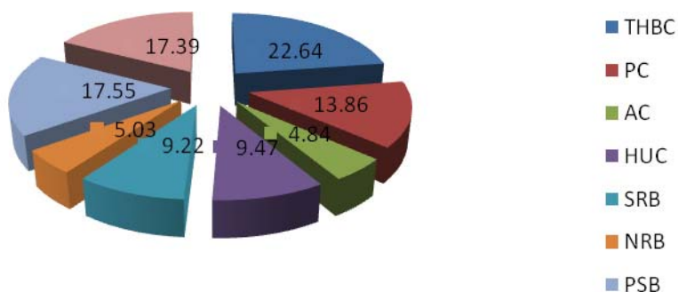
Figure 3: Abundance (%) of heterotrophic and autotrophic bacteria communities in the sediment samples during high tide Key: THB = Total heterotrophic bacteria, PC = Pseudomonas count, AC = Actinomycetes count, HUB = Hydrocarbon utilizing bacteria, FC = Fungal count, SRB = Sulphate reducing bacteria, NRB = Nitrate reducing bacteria, PSB = Phosphate solubilizing bacteria.
