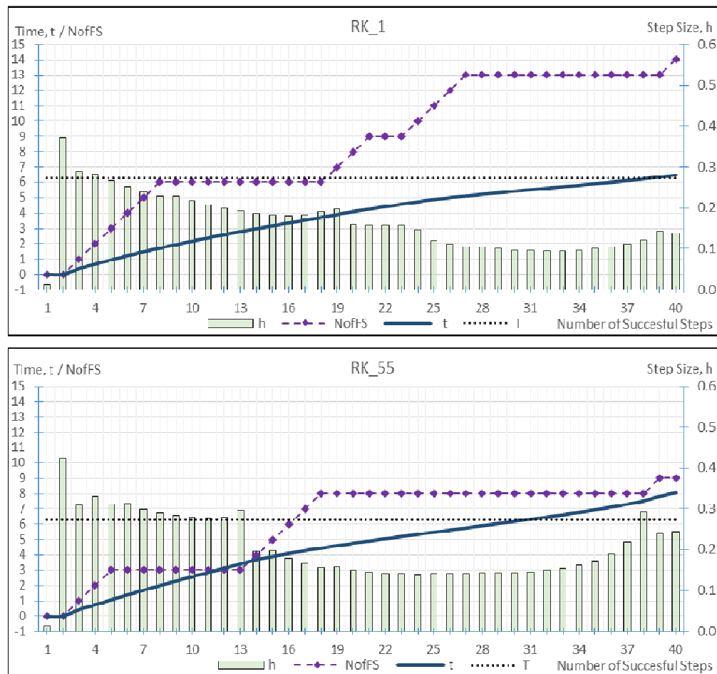
Fig. 3 Time series for a period of oscillation for the Duffing equation for two Runge Kutta versions. It shows the adaptive step size and number of failed steps (NofFS) for each step.
