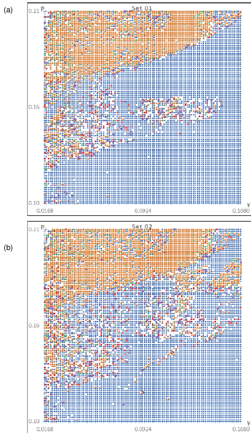
Fig. 4 Parameter plane highlighting the (five) versions with the lowest number of steps when used to simulate the dynamics of systems in (a) Set 1 (b) Set 2
