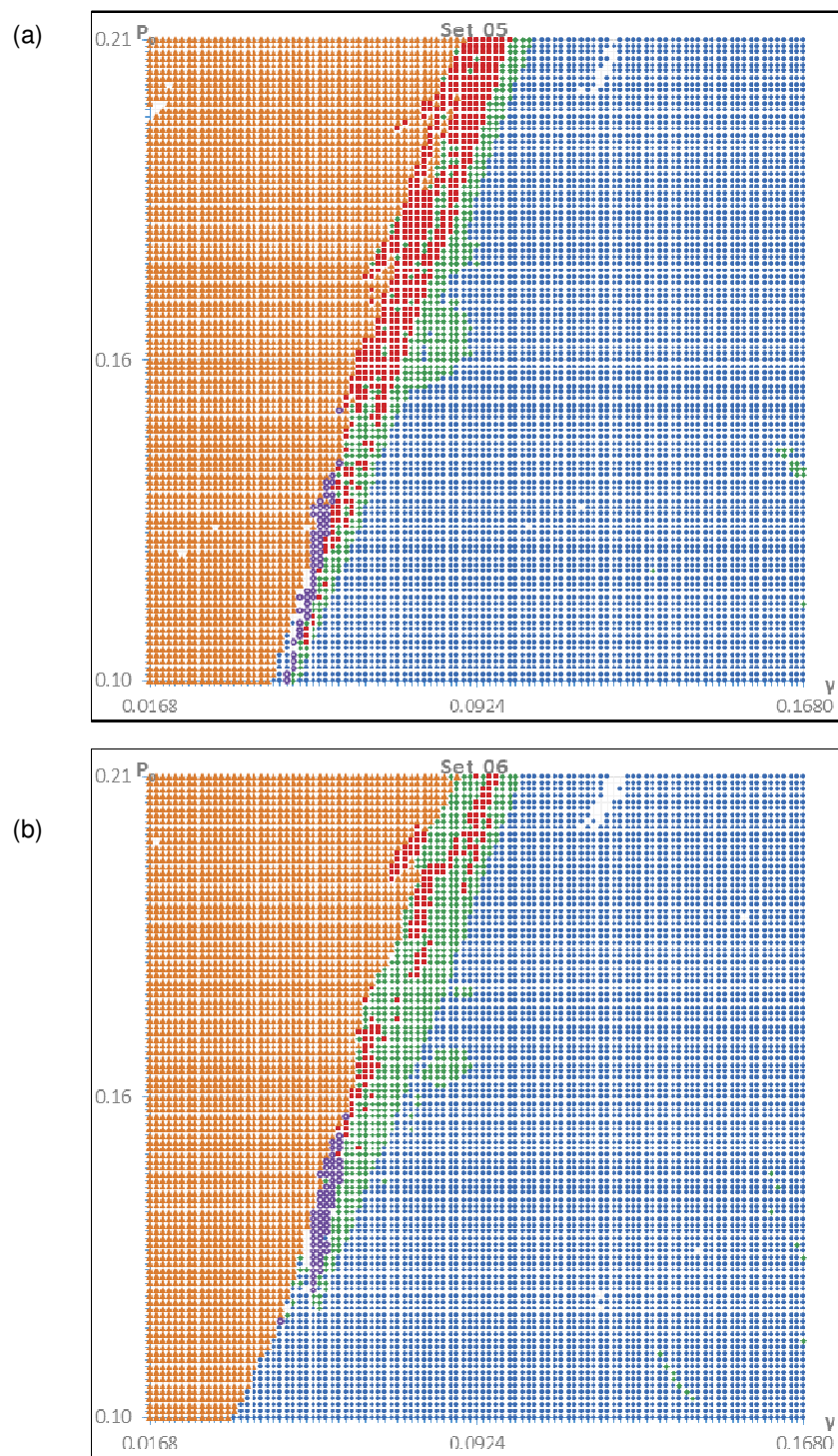
Fig. 6 Parameter plane highlighting the (five) versions with the lowest number of steps when used to simulate the dynamics of systems in (a) Set 5 (b) Set 6
