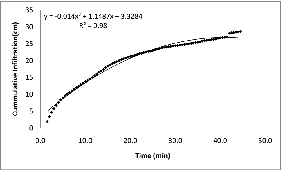
Figure 6: Cumulative Infiltration depth versus time in Plot C
