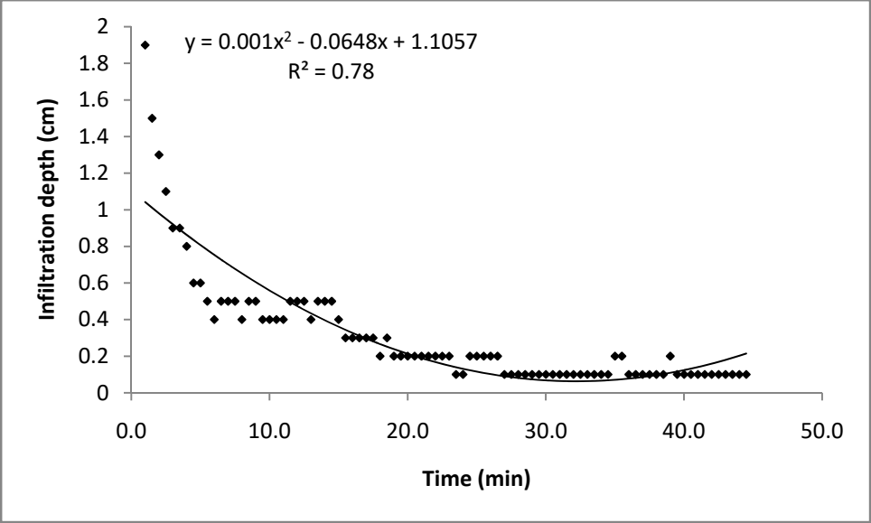
Figure 5: Infiltration depth versus time in Plot C
