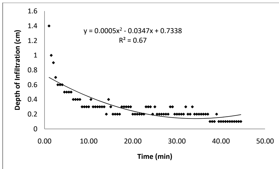
186 Figure 1: Infiltration depth versus time in Plot A
