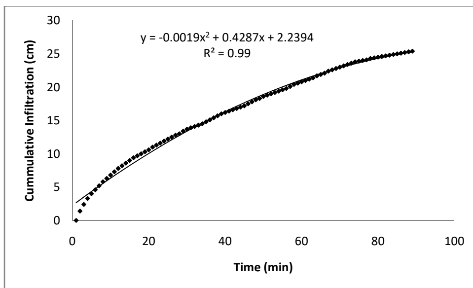
188 Figure 2: Cumulative Infiltration depth versus time in Plot A
