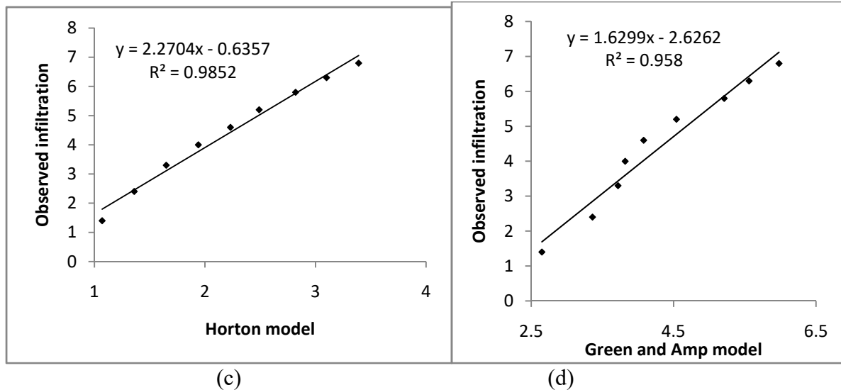
Figures 8 (a), (b), (c) and (d) Graph of predicted accumulated infiltration (cm) versus observed values.
