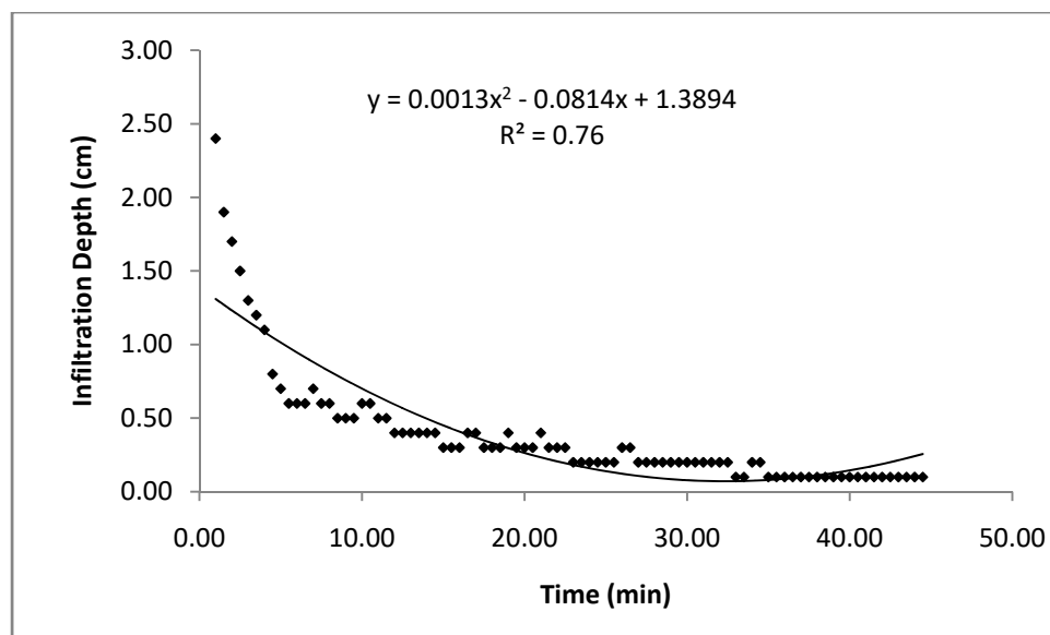
Figure 3: Infiltration depth versus time in Plot B
