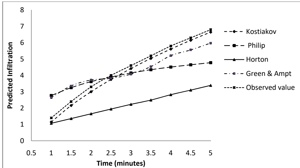
Figure 7 Graph of the predicted accumulated infiltration (cm) of the various models
