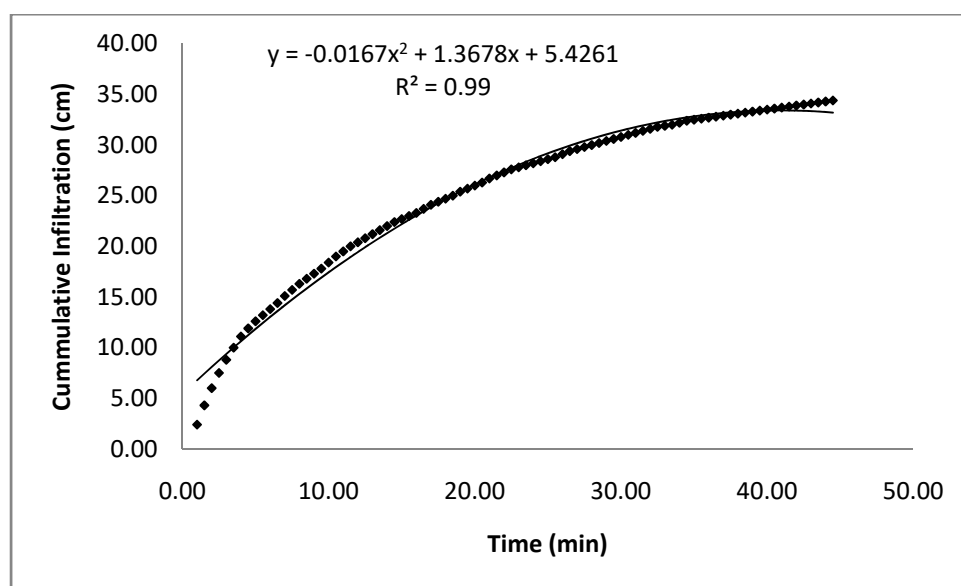
Figure 4: Cumulative Infiltration depth versus time in Plot B
