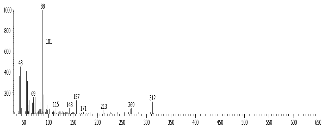
Figure 14: GC MS data base for like compound (octadecanoic acid ethyl ester)
