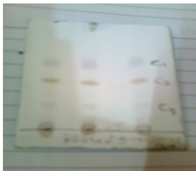
Figure 2: Separated and visualized spots of chloroform fraction
