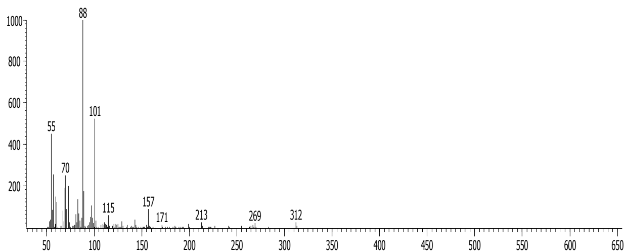
Figure 13: compound C2 GC MS data showing peaks
