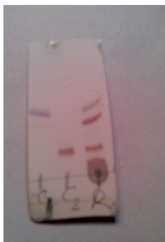
Figure 3: TLC of Pure compound C1 and C3 confirmed
