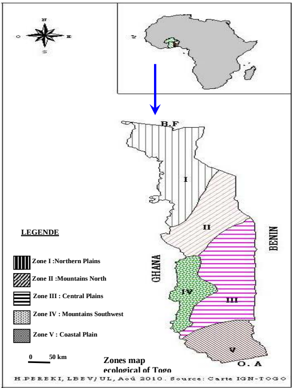
Fig. 1. Map of Ecological Zones of Togo (source: Koudégnan & al. (2014))
