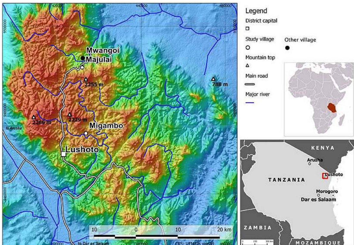
Fig. 1. Location map of Majulai and Migambo villages, Lushoto District, Tanzania. (Adapted from Msita, 2013)
