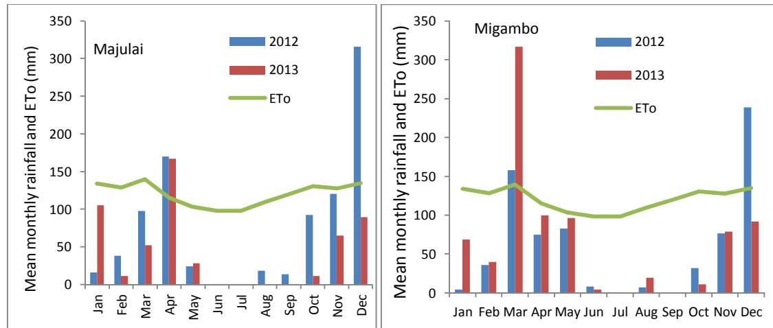
Fig. 3: Rainfall distribution in Majulai and Migambo villages and estimated reference evapo-transpiration (ET o ) measured during 2012 and 2013; ET o determined according to New_LocClim estimator; [19].
