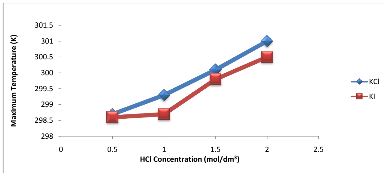
Figure 4. Variation of temperature with HCl concentration for the corrosion of zinc in 0.5M KCl and KI
