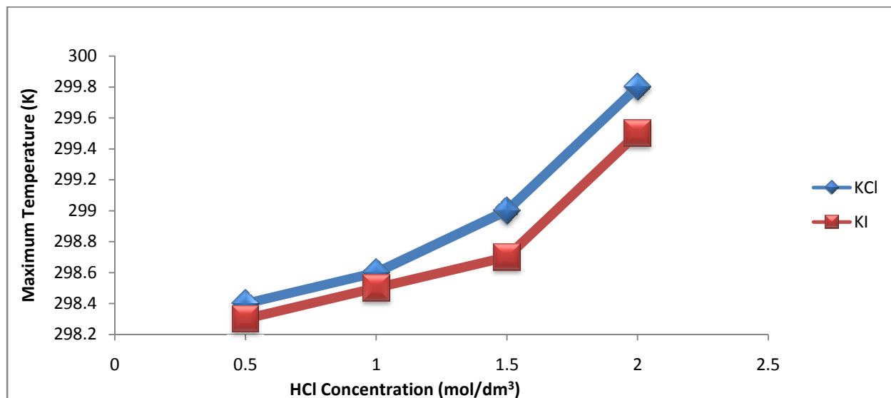
Figure 5. Variation of temperature with HCl concentration for the corrosion of zinc in 0.1M KCl and KI, and 0.3g/L inhibitor
