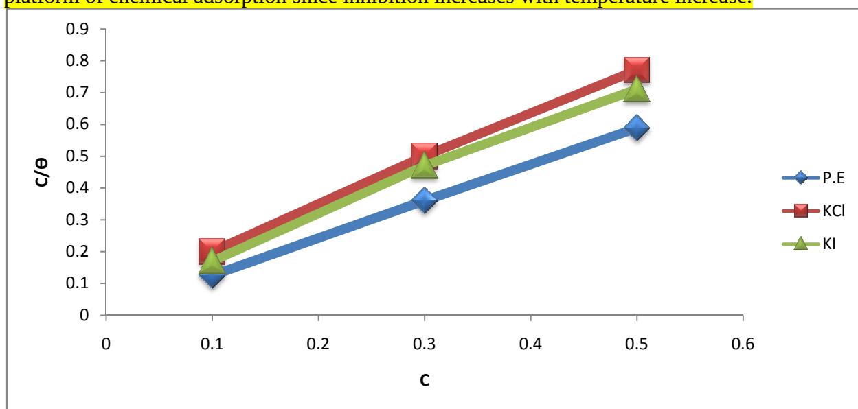
Figure 8: Langmuir isotherm model for the corrosion of zinc in varying plant extract, KCl and KI concentration at 1.5M HCl solution
