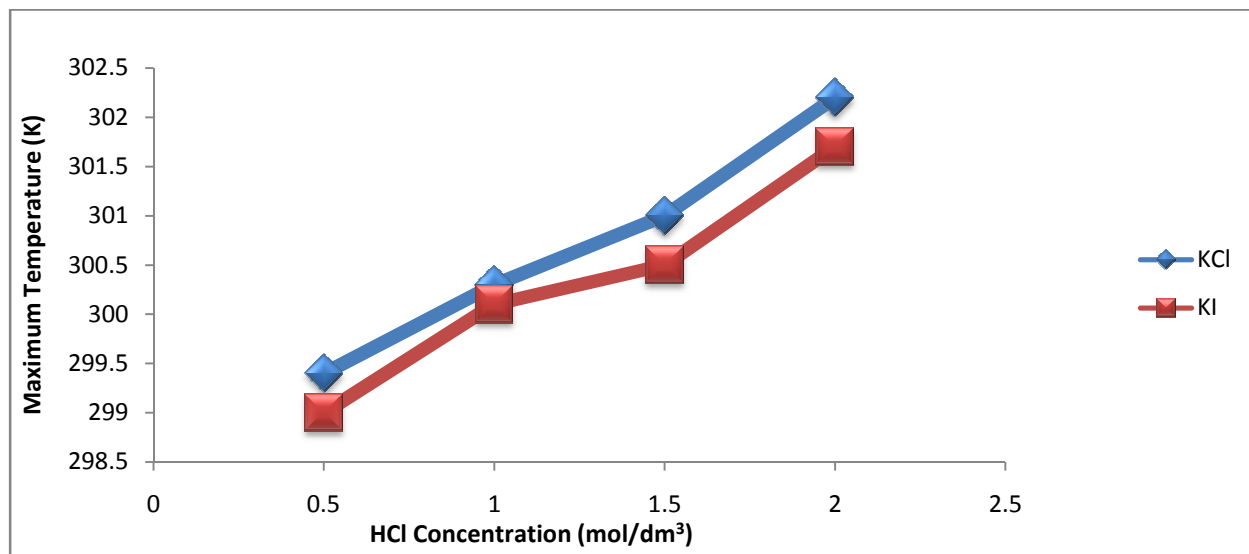
Figure 2. Variation of temperature with HCl concentration for the corrosion of zinc in 0.1M KCl and KI
