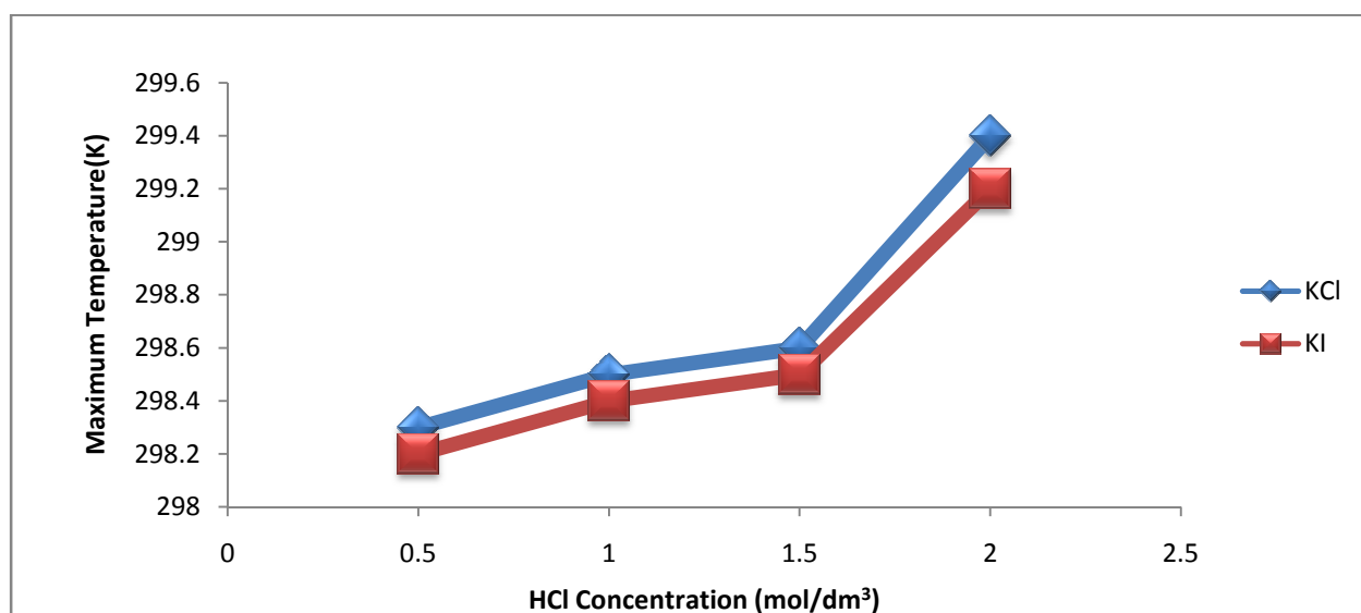
Figure 6. Variation of temperature with HCl concentration for the corrosion of zinc in 0.3M KCl and KI, and 0.3g/L inhibitor
