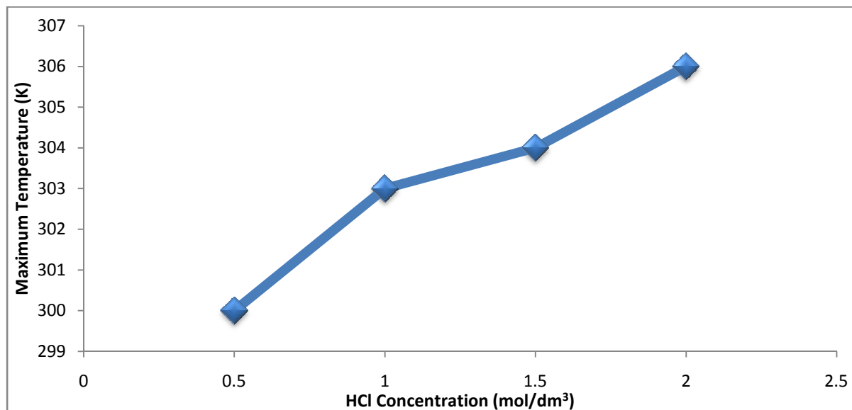
Figure 1. Variation of temperature with HCl concentration for the corrosion of Zinc
