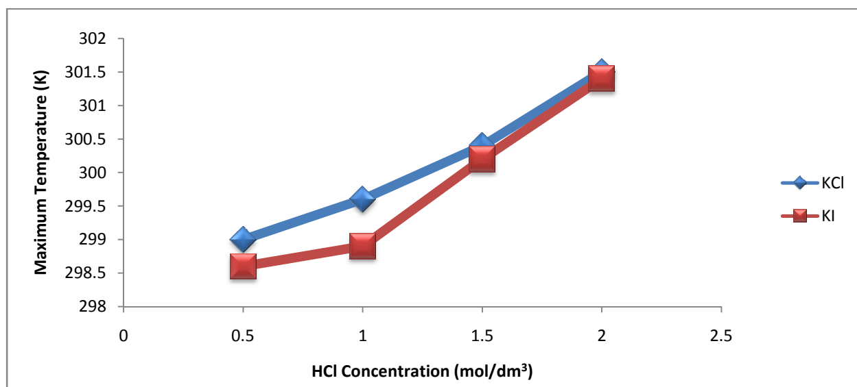
Figure 3. Variation of temperature with HCl concentration for the corrosion of zinc in 0.3M KCl and KI
