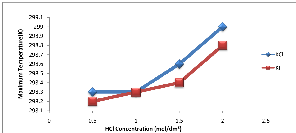
Figure 7. Variation of temperature with HCl concentration for the corrosion of zinc in 0.5M KCl and KI, and 0.3g/L inhibitor
