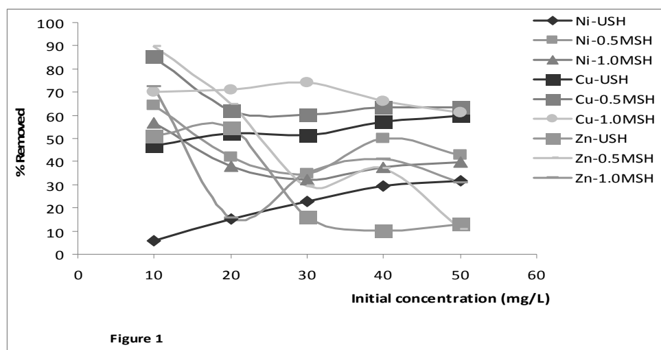
Figure 1: Percentage removed against Initial concentration of metal ion solution for 106 \mu\text{m}
