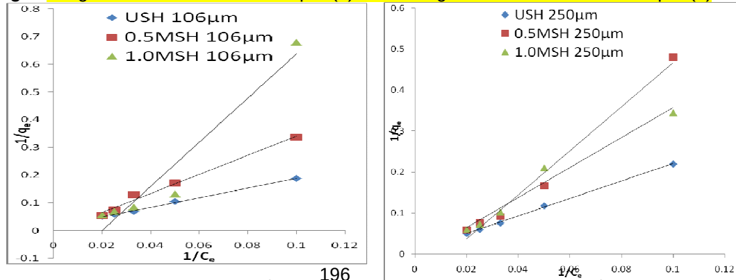
Fig.4: Langmuir isotherm for \text{Cu}^{2+} 106µm (a) Langmuir isotherm for \text{Cu}^{2+} 250µm (b)
