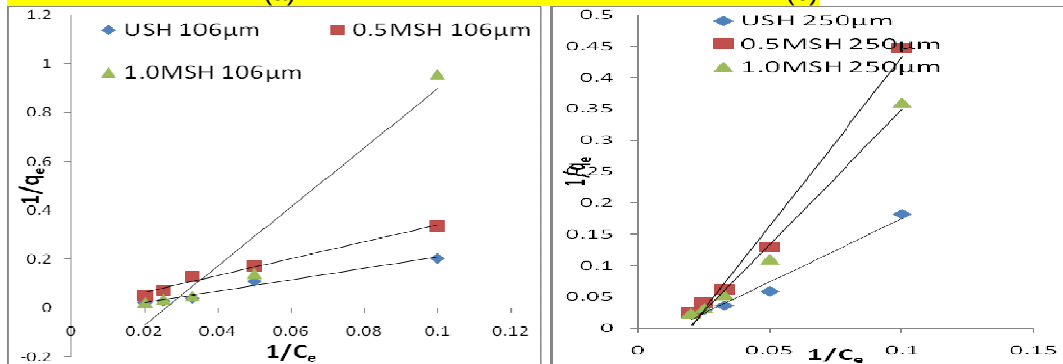
Fig.5: Langmuir isotherm for \text{Zn}^{2+} 106µm (a) Langmuir isotherm for \text{Zn}^{2+} 250µm (b)
