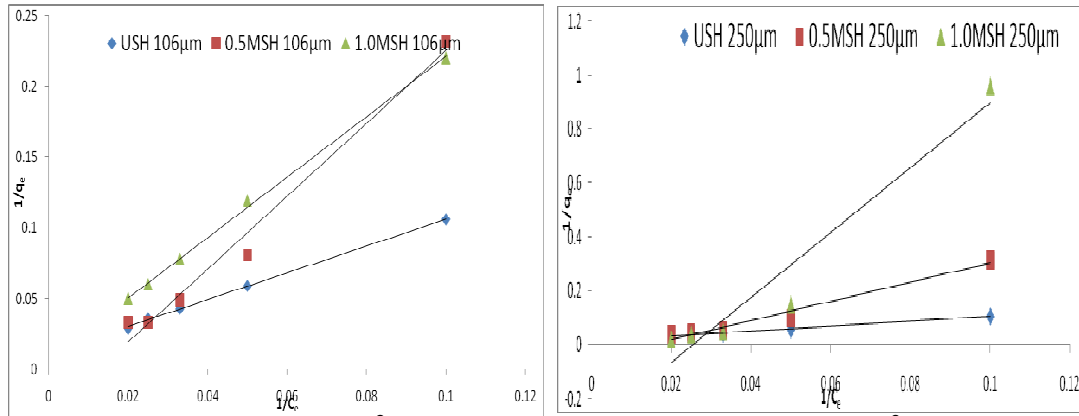
Fig 3: Langmuir isotherm for \text{Ni}^{2+} 106µm (a) Langmuir isotherm for \text{Ni}^{2+} 250µm (b)
