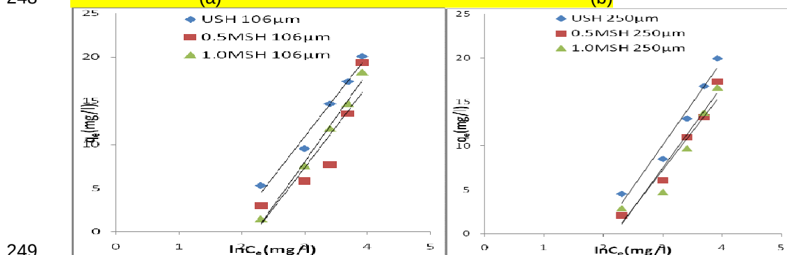
Fig. 10: Temkin isotherm for \text{Cu}^{2+} 106µm (a) Temkin isotherm for \text{Cu}^{2+} 250µm. (b)
