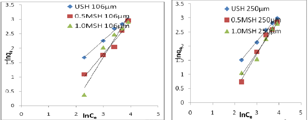
219 Fig.7: Freundlich isotherm for \text{Cu}^{2+} 220 106 \mu\text{m} (a) 221 250 \mu\text{m} (b)
