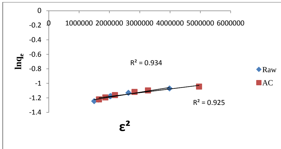
Figure 7. Dubinin-Radushkevich isotherms plot for adsorption of copper ion onto raw and activated adsorbents
