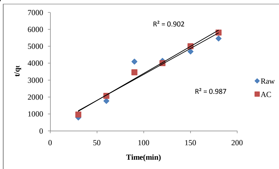
Figure 10. Pseudo-second-order plot for adsorption of copper ion onto raw and activated adsorbents
