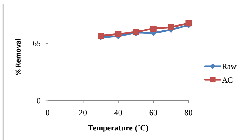
Figure 5. Effect of temperature on the removal of copper ion by adsorption at 5\text{mgdm}^{-3} concentration, contact time 90min and pH 6.9
