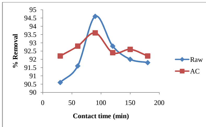
Figure 1. Effect of contact time on the removal of copper ion by adsorption at 5\text{mgdm}^{-3} , 0.5\text{g} adsorbents weight, pH 6.9 and temperature 28^\circ\text{C} \pm 1
