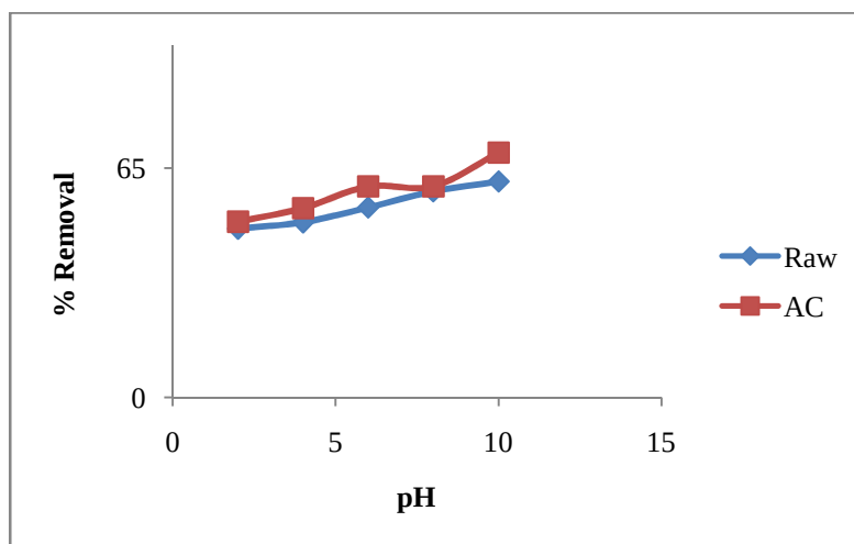
Figure 2. Effect of pH on the removal of copper ion by adsorption at 5\text{mgdm}^{-3} concentration and 0.5g adsorbents weight
