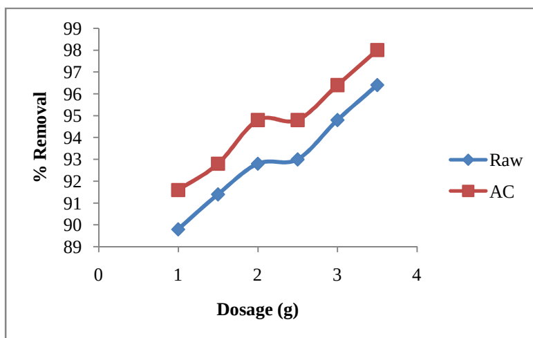
Figure 4. Effect of adsorbent dose on the removal of copper ion by adsorption at contact time 90min, 5\text{mgdm}^{-3} concentration and pH 6.9
