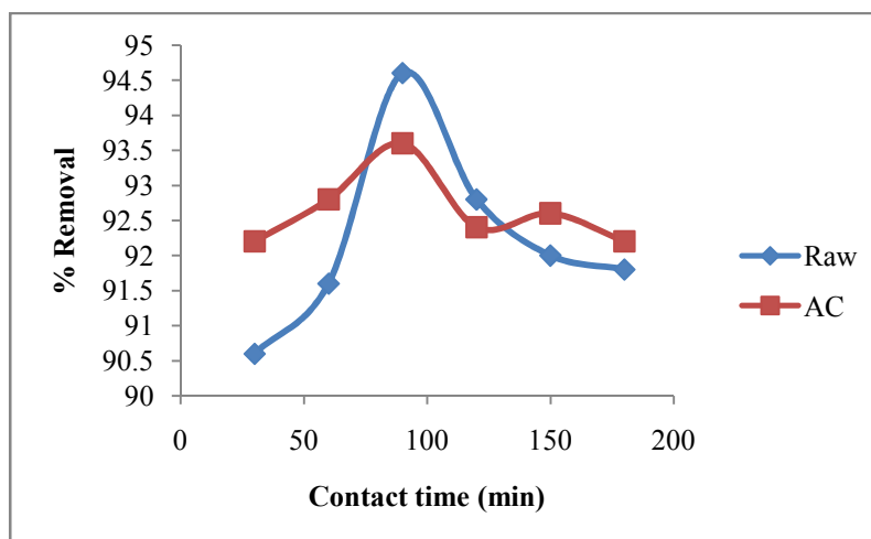
Figure 1. Effect of contact time on the removal of copper metal by adsorption at 5\text{mgdm}^{-3} , 0.5\text{g} adsorbents weight and temperature 28^{\circ}\text{C} \pm 1
