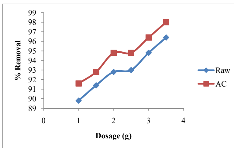
Figure 4. Effect of adsorbent dose on the removal of copper metal by adsorption at 5\text{mgdm}^{-3}
