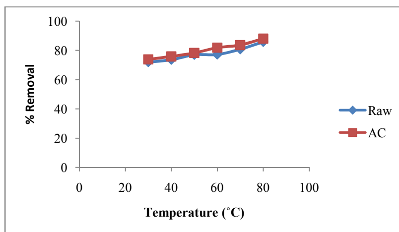
Figure 5. Effect of temperature on the removal of copper metal by adsorption at 5\text{mgdm}^{-3}
