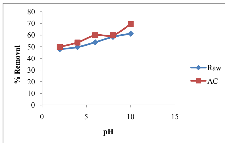
Figure 2. Effect of pH on the removal of copper metal by adsorption at 5\text{mgdm}^{-3} and 0.5\text{g} adsorbents weight
