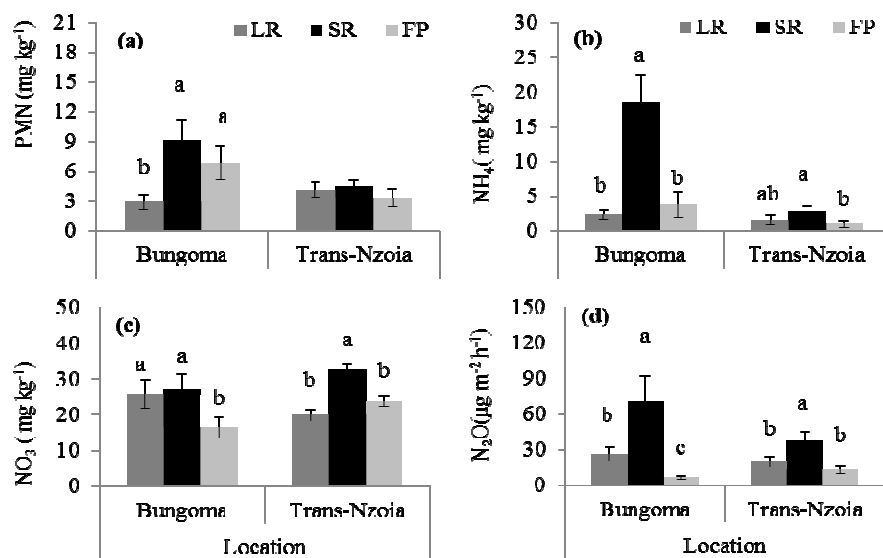
Fig. 4. (a) Soil potentially mineralizable nitrogen (PMN), (b) ammonium (NH 4 ), (c) nitrate (NO 3 ) concentrations and (d) nitrous oxide (N 2 O) fluxes for long rains (LR), short rains (SR) and Fallow Period (FP) for Bungoma and Trans-Nzoia locations. Lower case letters indicate least significant differences at P \leq 0.05
