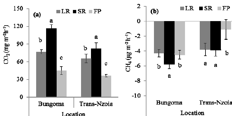
Fig. 6. (a) Carbon dioxide ( CO_2 ) and (b) methane ( CH_4 ) fluxes during short rains (SR), fallow period (FP) and long rains (LR) averaged across the three years Bungoma and Trans-Nzoia locations. Lower case letters indicate least significant differences at P \leq 0.05
