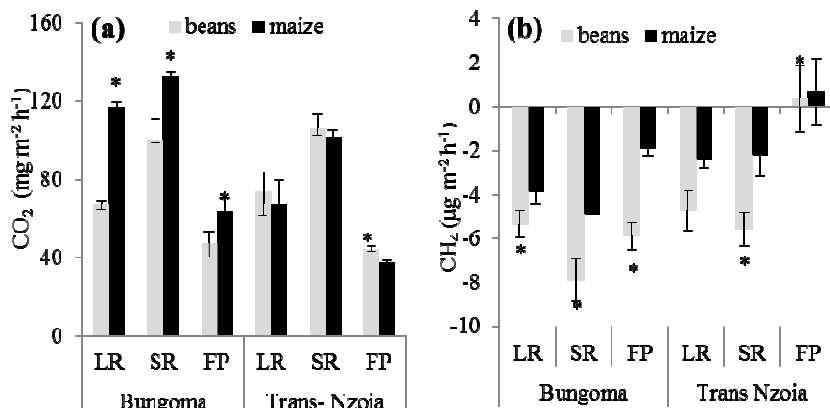
Fig. 7. (a) Carbon dioxide ( CO_2 ) and (b) methane ( CH_4 ) from soils associated with different crops (beans and maize) during long rains (LR), short rains (SR) and fallow period (FP) at Bungoma and high Trans-Nzoia locations averaged across the three years. Asterisks indicate a significant difference between crops at P \leq 0.05 within each location
