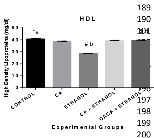
201 Figure 3: Effect of different treatments on the High Density Lipoproteins levels in the Serum of 202 rats.
