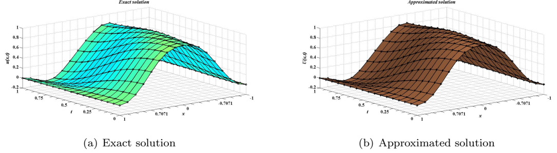
FIGURE 1. Exact and Approximated solutions for p(x) with x \in [-1, 1] and t \in [0, T] at N = 16 . See Example 3.1.
