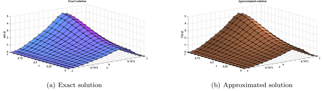
FIGURE 2. Exact and Approximated solutions for p(x) with x \in [-1, 1] and t \in [0, T] at N = 18 . See Example 3.2.
