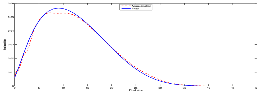
Figure 1: Distribution of the final size and its diffusion approximation, for n = 50 , m = 10 , \beta = 0.2 , \mu = 0.1 .
