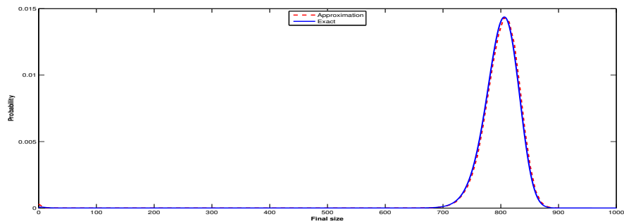
Figure 6: Distribution of the final size and its diffusion approximation, for n = 1000 , m = 10 , \beta = 0.2 , \mu = 0.1 .
