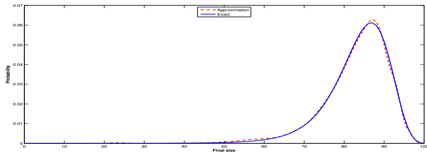
Figure 4: Distribution of the final size and its diffusion approximation, for n = 100 , m = 10 , \beta = 0.2 , \mu = 0.3 .
