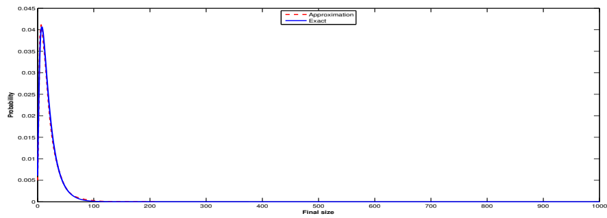
Figure 5: Distribution of the final size and its diffusion approximation, for n = 1000 , m = 10 , \beta = 0.2 , \mu = 0.3 .
