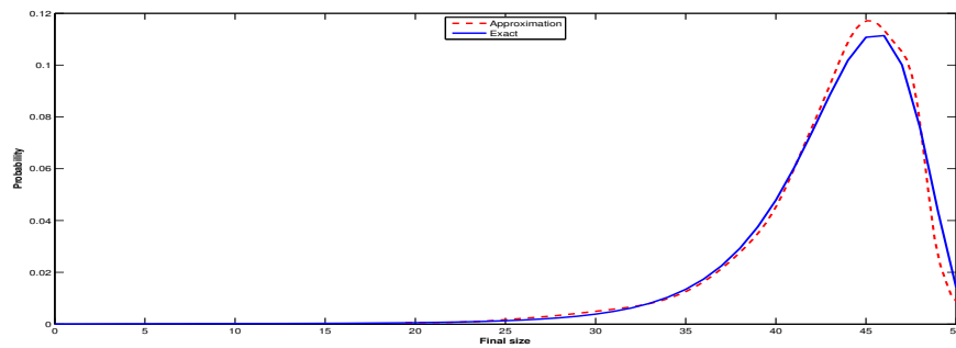
Figure 2: Distribution of the final size and its diffusion approximation, for n = 50 , m = 10 , \beta = 0.2 , \mu = 0.1 .
