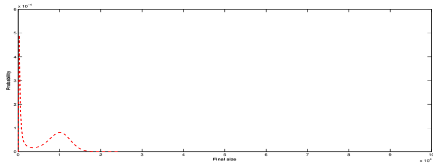
Figure 8: Distribution of the final size by diffusion approximation, for n = 10^6 , m = 10 , \beta = 0.2 , \mu = 0.1 .
