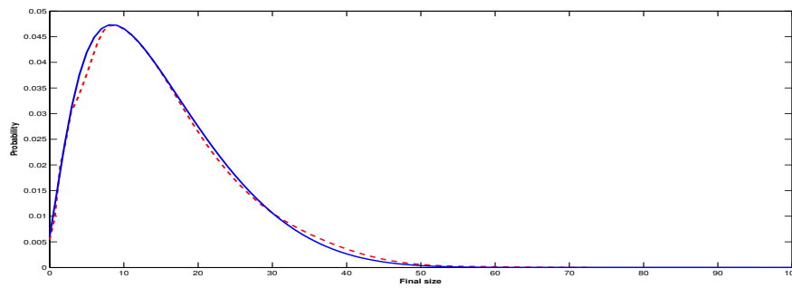
Figure 3: Distribution of the final size and its diffusion approximation, for n = 100 , m = 10 , \beta = 0.2 , \mu = 0.1 .
