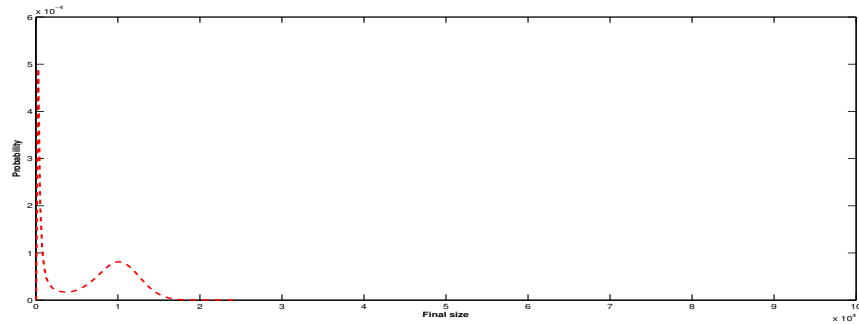
Figure 7: Distribution of the final size by diffusion approximation, for n = 10^5 , m = 10 , \beta = 0.2 , \mu = 0.1 .
