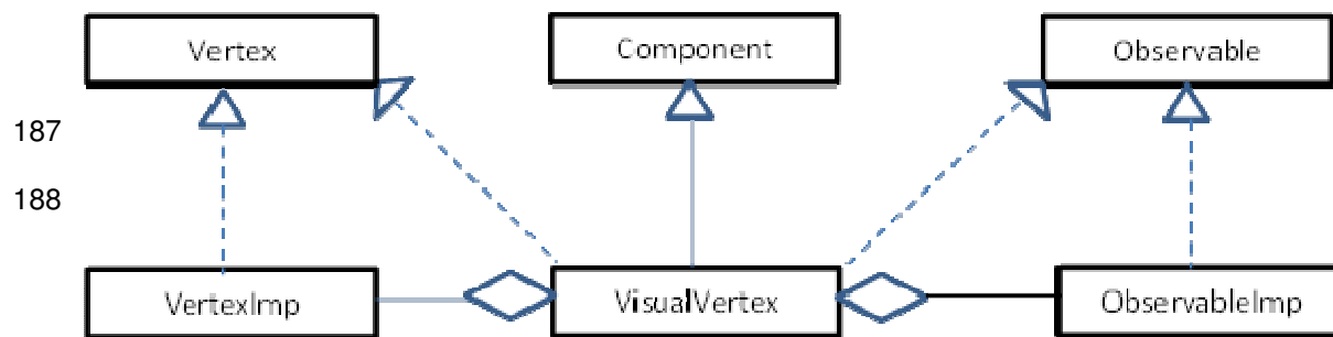
Figure 3-2 Java-Oriented Design
