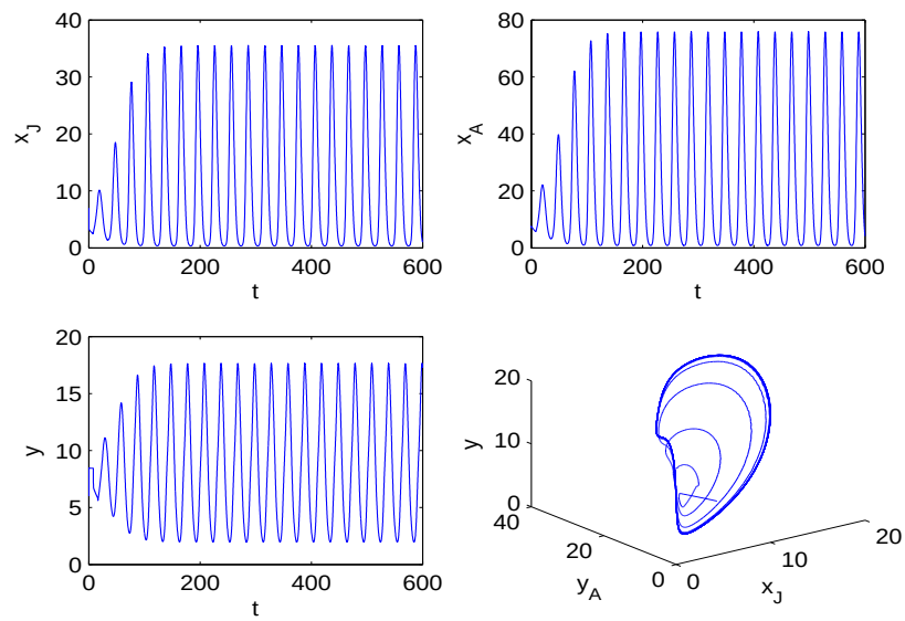
Figure 2. Numerical simulations of a periodic solution to system (5.1) when \tau = 8 > \tau_0 = 7.4421 .
