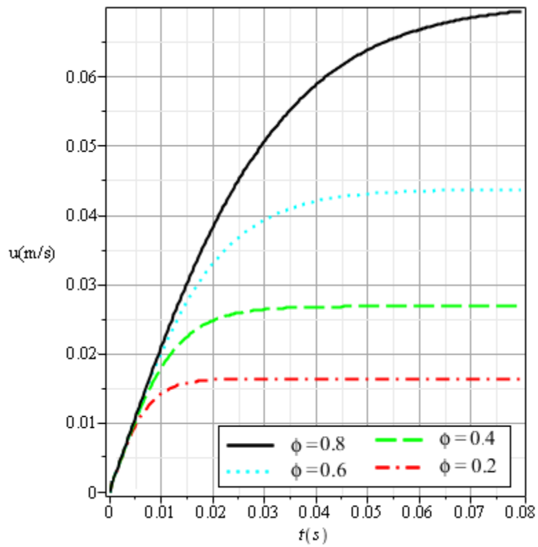
Fig. 6. Velocity profiles of different solid sphericity used in Water.
