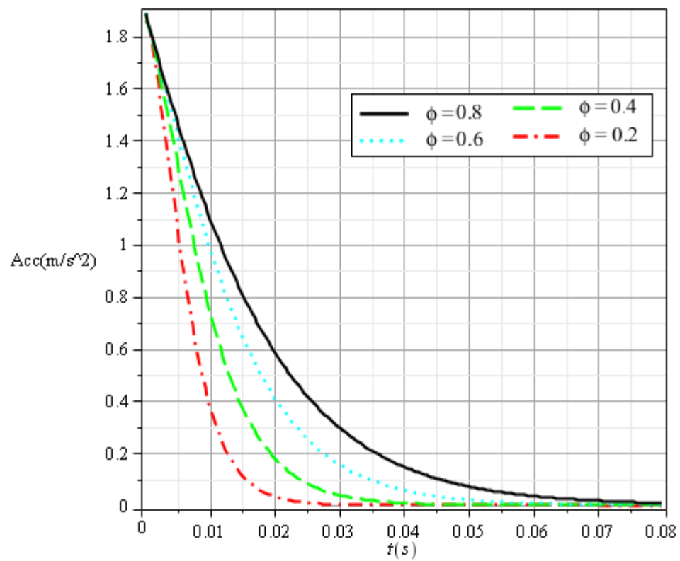
Fig. 8. Acceleration profiles of different solid spherecity used in Ethylene glycol.
