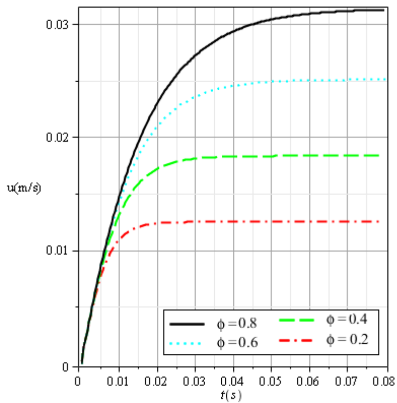
Fig. 5. Velocity profiles of different solid spherecity used in Ethylene glycol.
