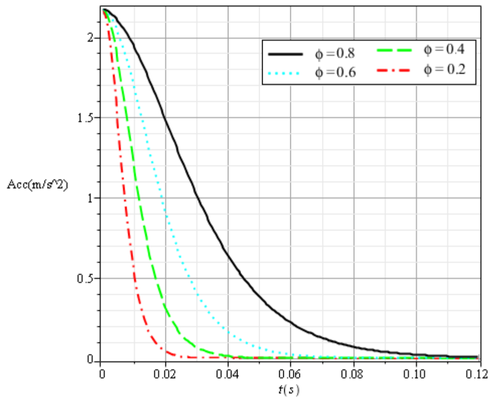
Fig. 7. Acceleration profiles of different solid spherecity used in Water.
