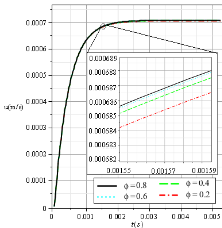
Fig. 4. Velocity profiles of different solid sphericity used in Glycerin.
