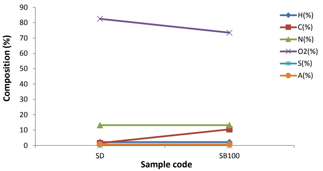
Figure 6: The relationship between briquetting on the ultimate analysis of sawdust
