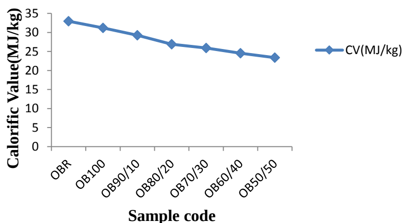
Figure 8: The effect of blending/briquetting on the calorific value of Okaba coal deposit
