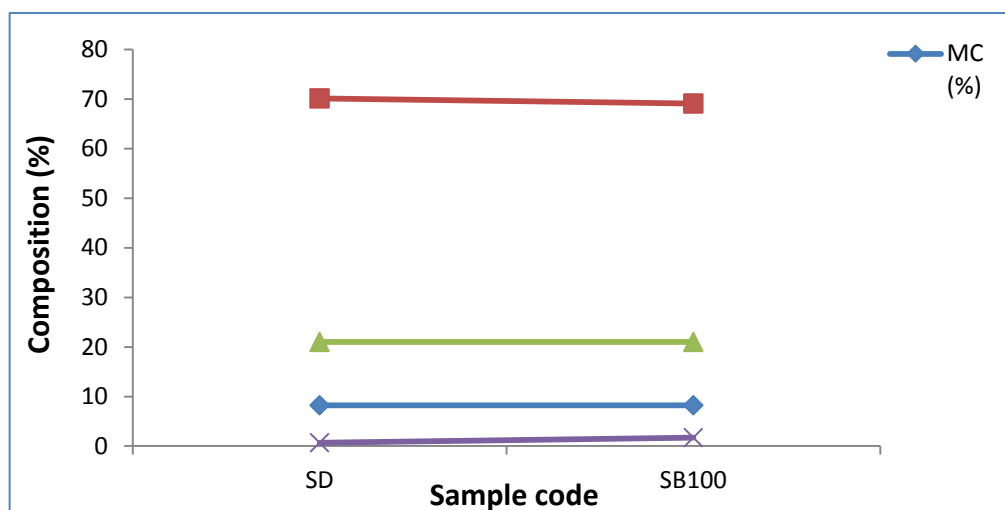
Figure 3: The relationship between blending and briquetting on the proximate analysis of sawdust
