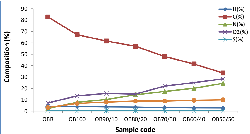
Figure 5: The relationship between blending/briquetting on the ultimate analysis of Okaba deposit
