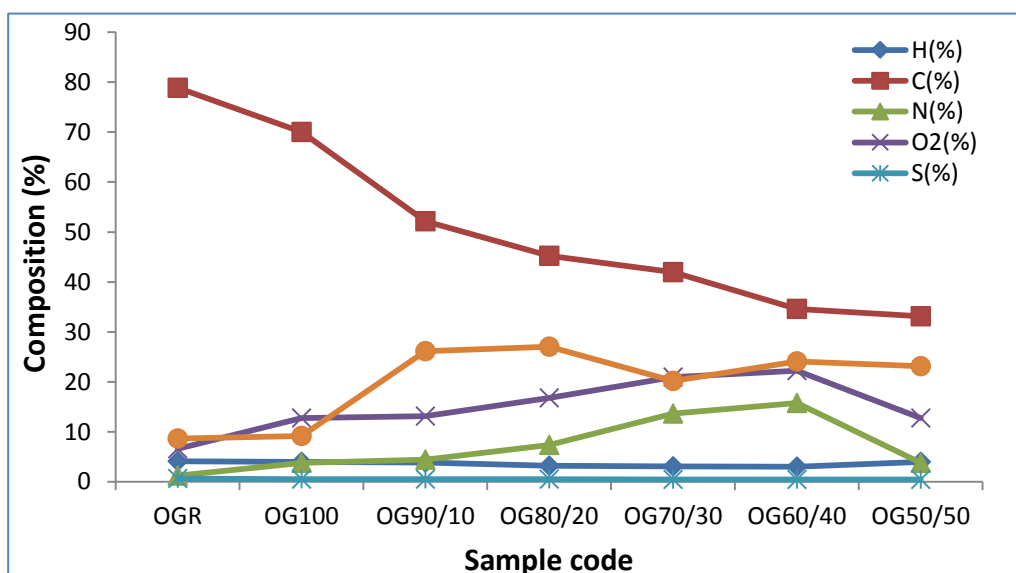
Figure 4: The relationship between blending and briquetting on the ultimate analysis of Ogboyaga(Odu) deposit
