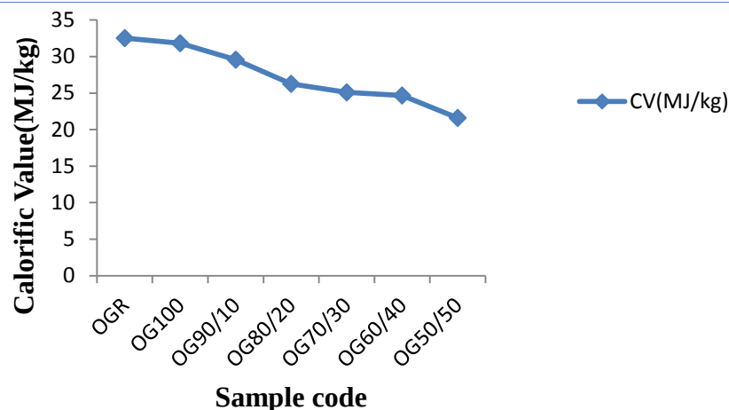
Figure7: The effect of blending/briquetting on the calorific value of Ogboyaga(Odu) deposit
