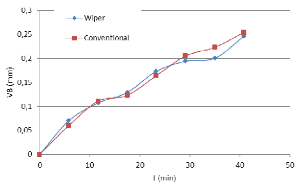
Figure 4 Graph of the cutting tool wear dependency on cutting time
