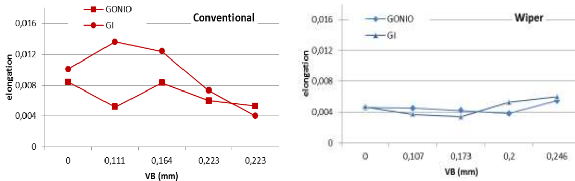
Figure 7 Influence of the flank wear on the elongation
