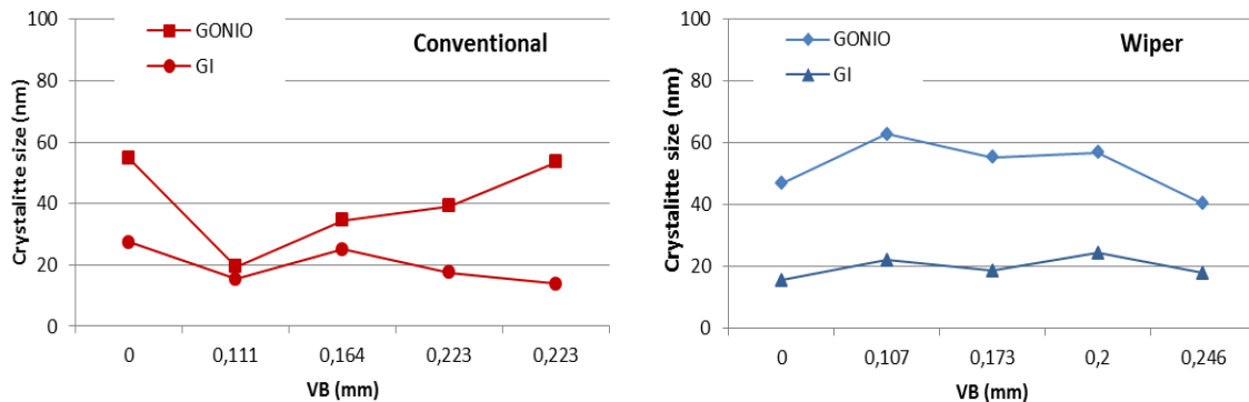
Figure 6 Crystallite size influenced by the flank wear VB
