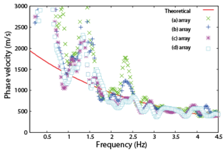
Fig. 9. Estimation from 4 linear arrays with different direction in a moderately azimuth-dependent wavefield
