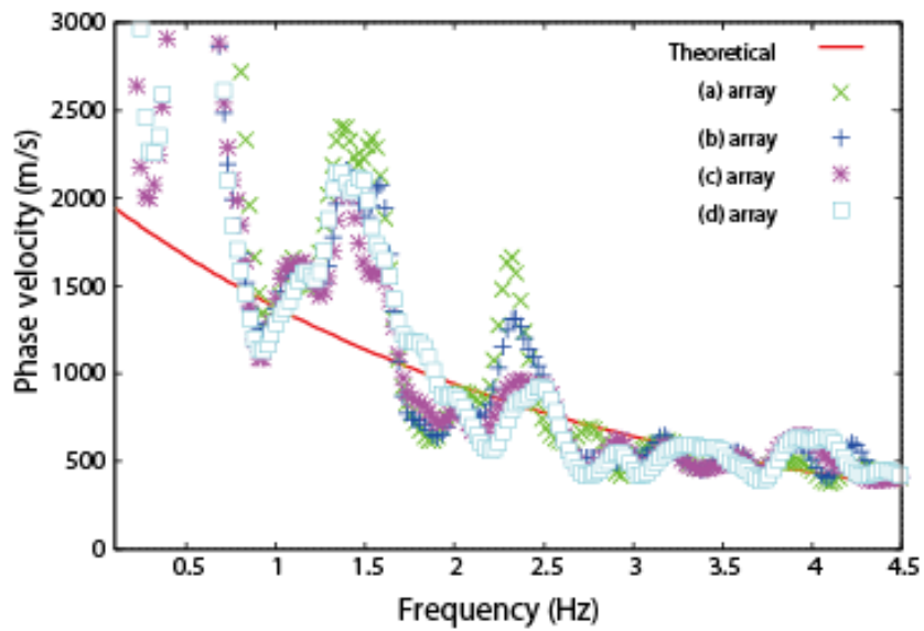
Fig. 8. Estimation from 4 linear arrays with different direction in an isotropic wavefield
