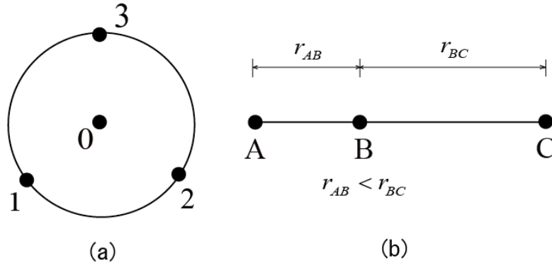
110 Fig. 2. Sensor arrangement of SPAC method and the new method (a) The equilateral 111 array used by SPAC method (b) The linear array with 3 sites on it 112
