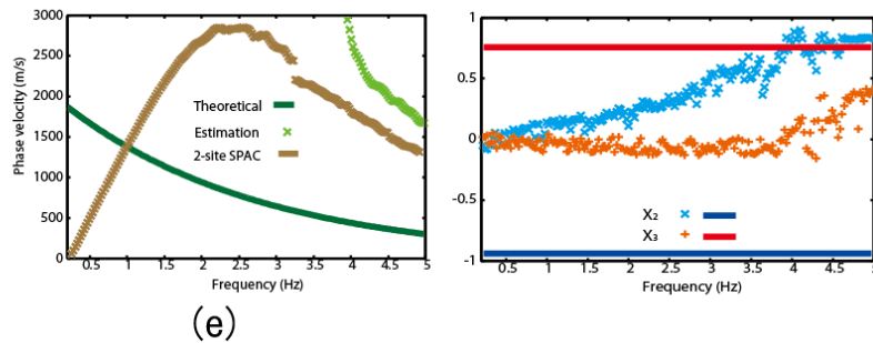
Fig. 4. Estimation of phase velocity, x_2 and x_3 in case of uni-directional plane wave with different direction. (a) 0^\circ (b) 30^\circ (c) 45^\circ (d) 60^\circ (e) 80^\circ .
