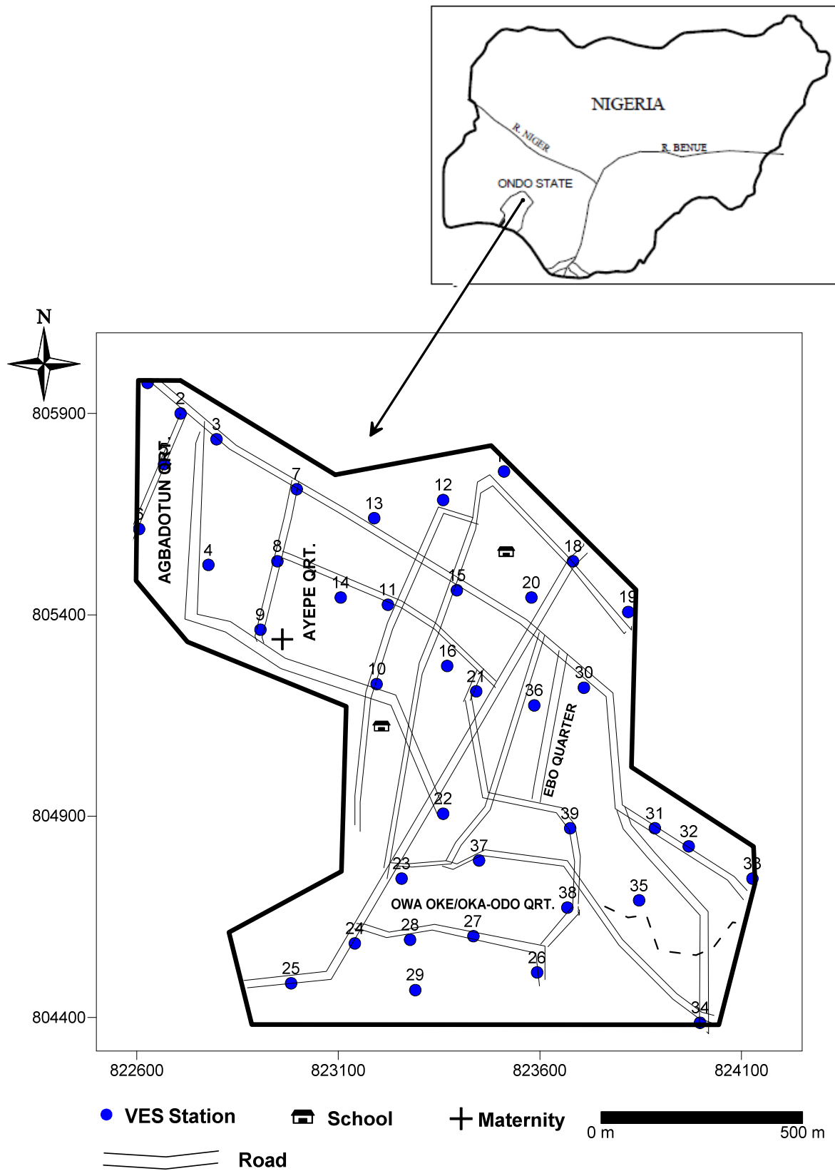
Fig. 1: Base Map of the Study Area Showing the Vertical Electrical Sounding (VES) Stations
