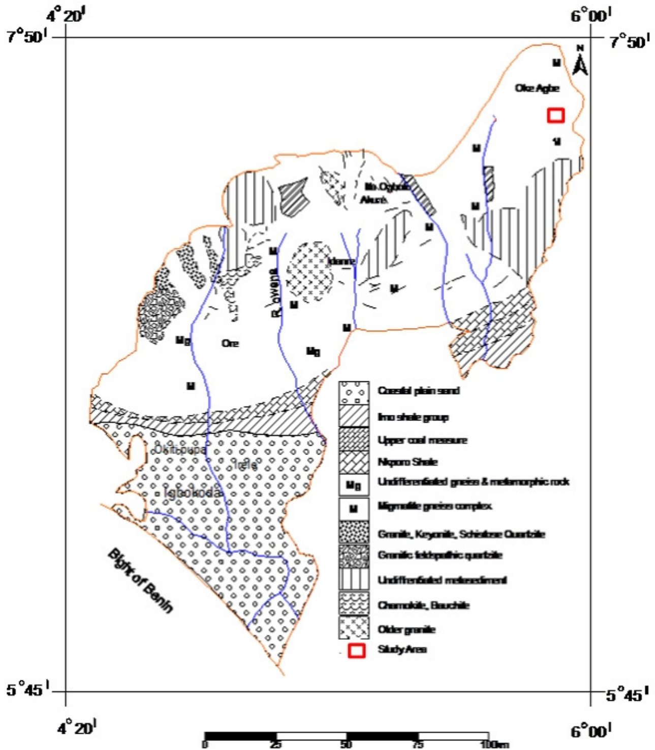
Fig. 2: Geological Map of Ondo State Showing the Study Area
