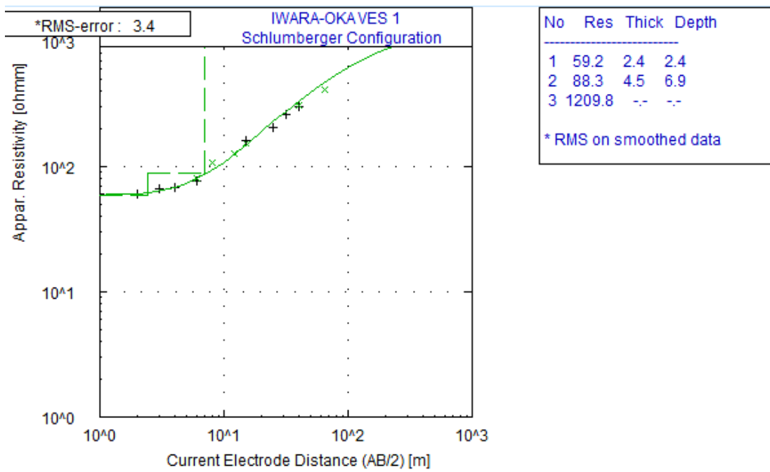
Fig. 4a: Typical Class 1 Type Curve
