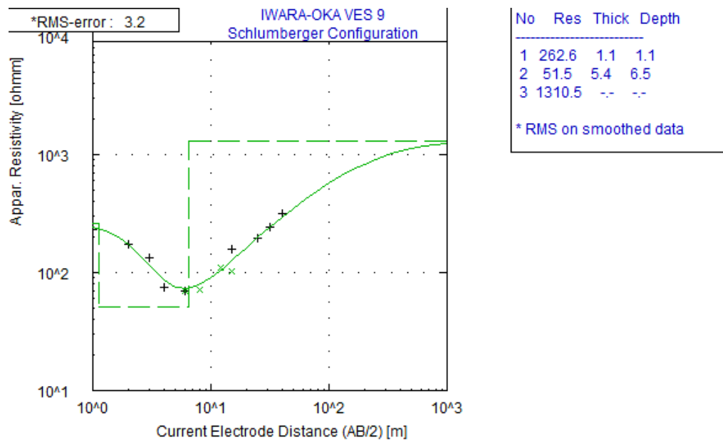
Fig. 4b: Typical Class 2 Type Curve
