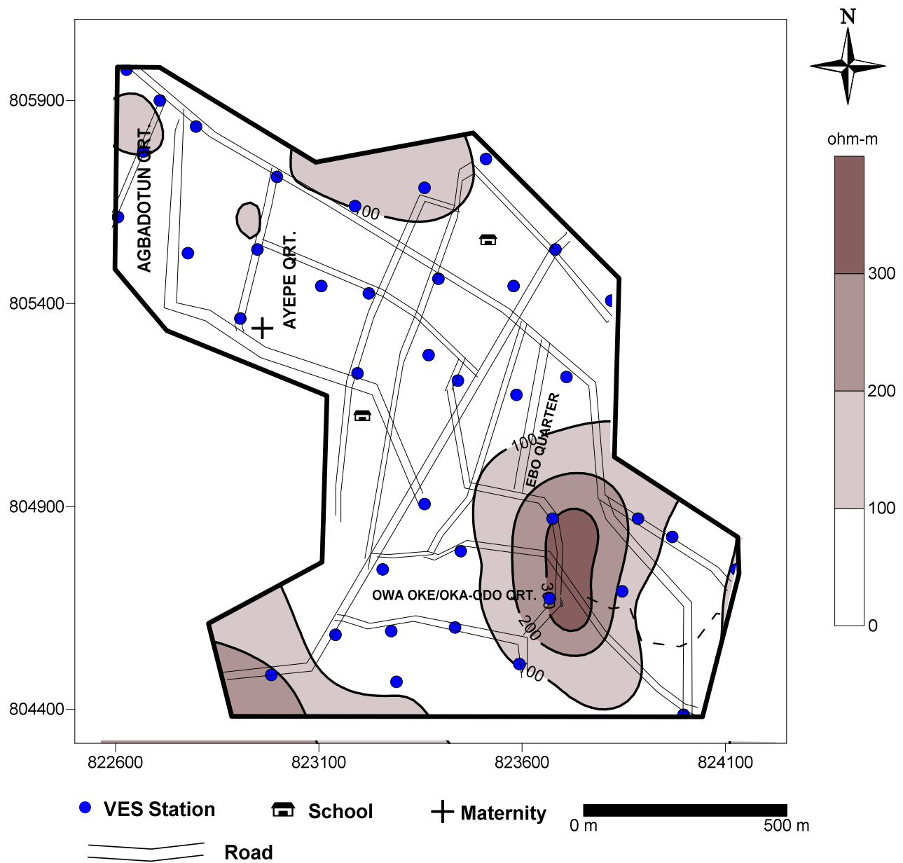
Fig. 6b: Isoresistivity Map of the Weathered Layer Aquifer Unit in the Study Area
